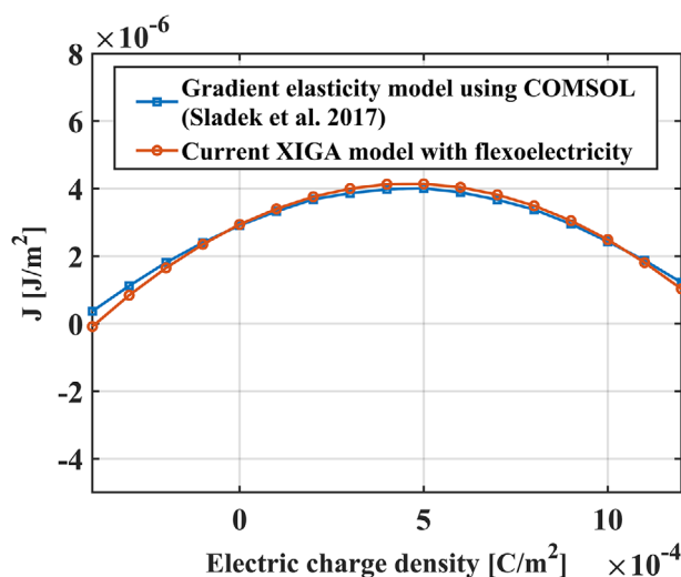
Figure 5. Validation of present XIGA model with flexoelectricity by comparing with previous publication; Sladek et al. 2017. [55]
