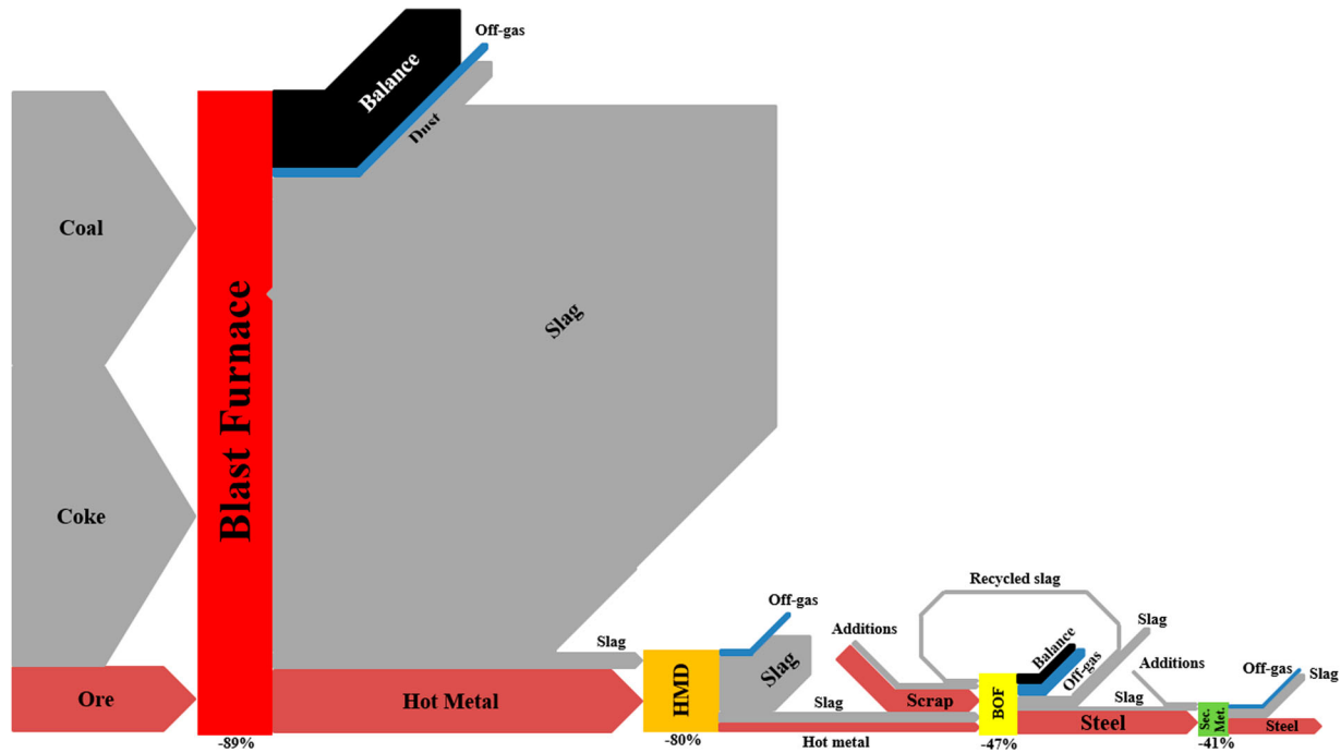
Figure 2. Sankey-type diagram of the sulphur distribution flow for a standard steel grade at Tata Steel IJmuiden in 2015. Arrows represent the amount of sulphur present in a flow, necessary for one tonne of produced steel. Below the process blocks the percentage of sulphur input that is removed in that process step is indicated.
