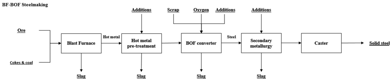
Figure 1. Block scheme of the BF-BOF steelmaking process.
