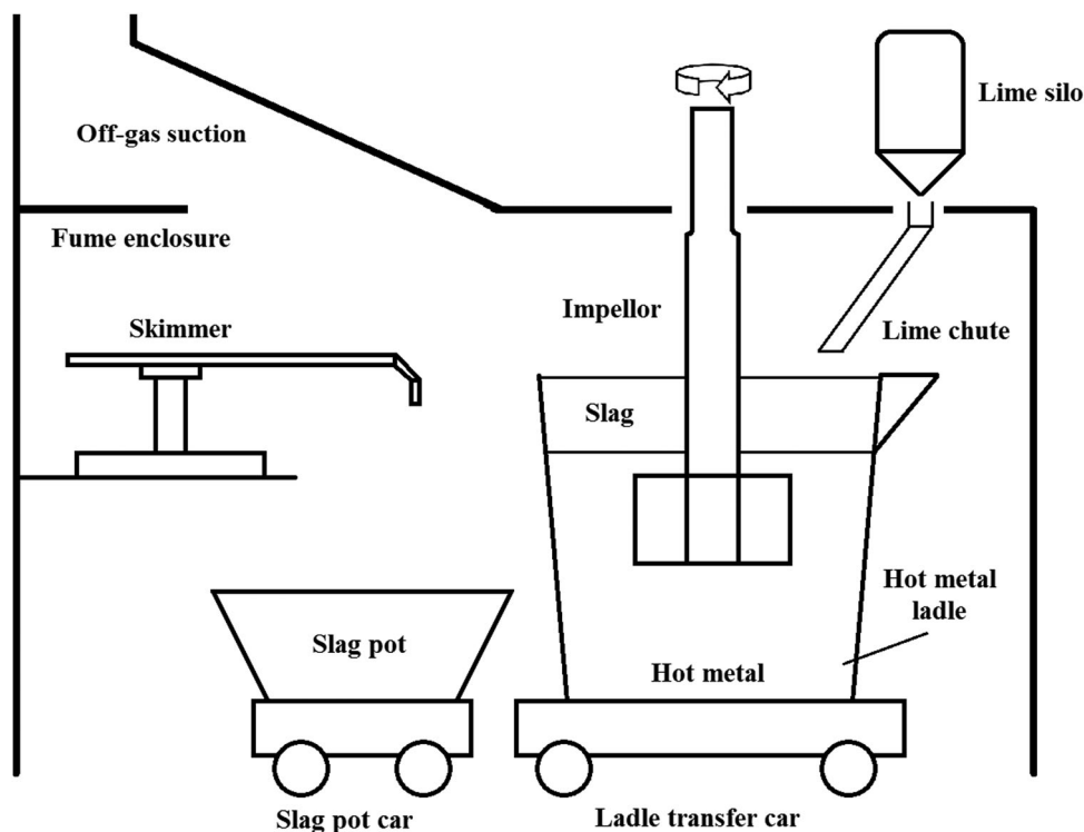
Figure 8. Schematic overview of a KR.
