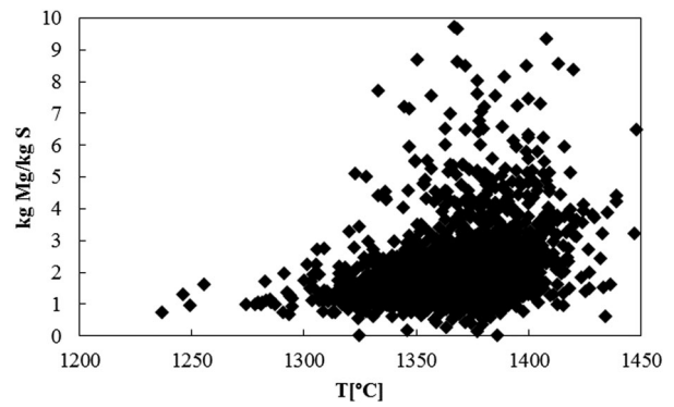
Figure 4. Amount of Mg used to remove 1 kg of sulphur at different HM temperatures. Data of 2158 heats at the HMD in a South American plant.
