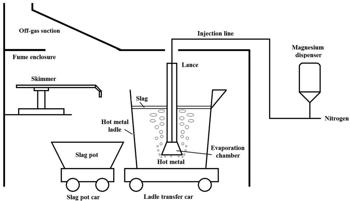
Figure 9. Schematic overview of MMI desulphurisation.
