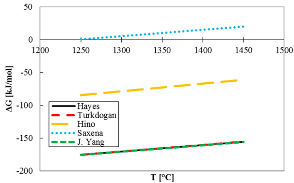
Figure 5. Temperature dependence of \Delta G^0 for the reaction between [Mg] and [S] (reaction 7), according to the literature.
