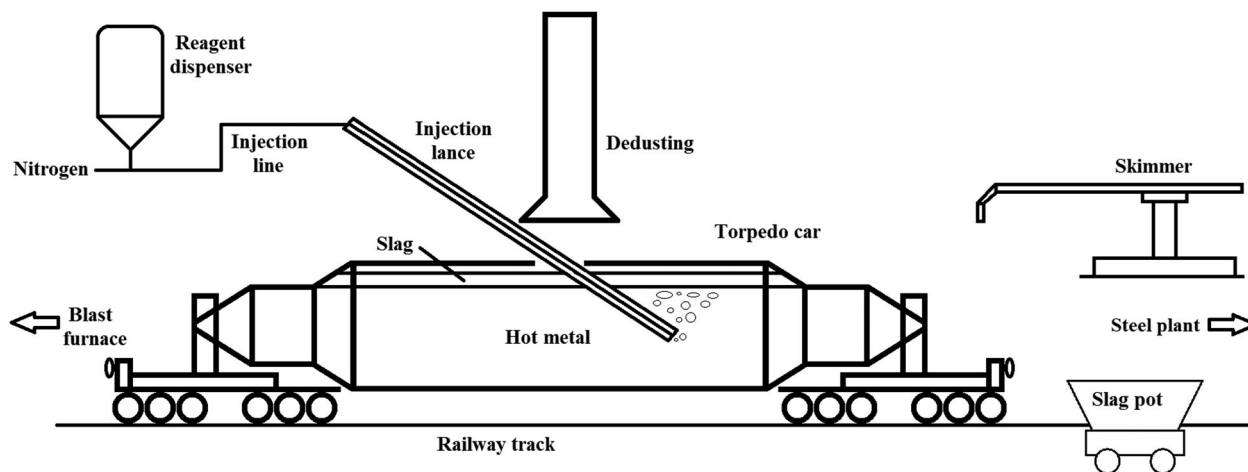
Figure 6. Schematic overview of torpedo desulphurisation.
