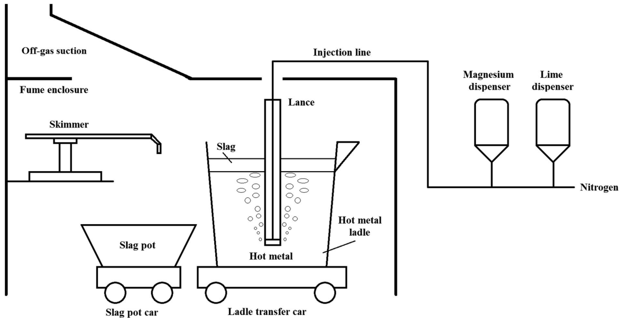
Figure 7. Schematic overview of co-injection desulphurisation.
