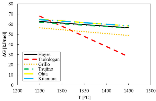
Figure 3. Temperature dependence of \Delta G^0 for the reaction between CaO and [S] (reaction 3), according to the literature.
