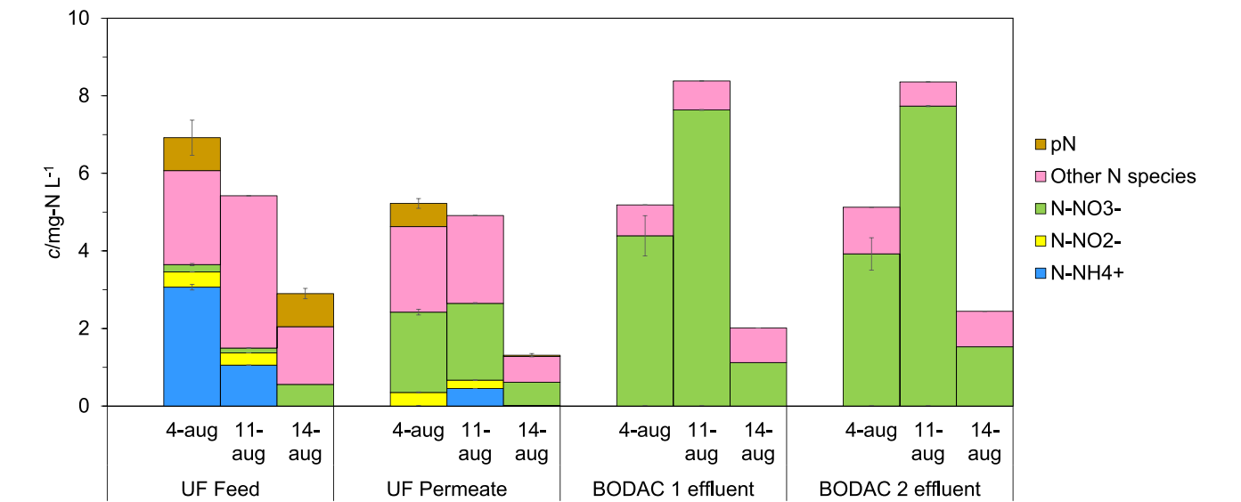
Fig. 4. The concentration of N species ( \text{N-NH}_4^+ , \text{N-NO}_2^- , \text{N-NO}_3^- , other N species) in the UPW plant, for three independent sampling days and triplicate samples were taken for each sampling point.
