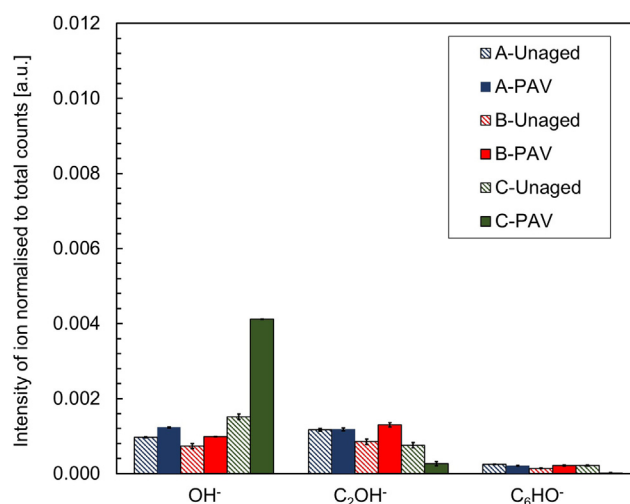
Fig. 12. Intensity of (\text{OH})_x -containing compounds in all the ageing states.
