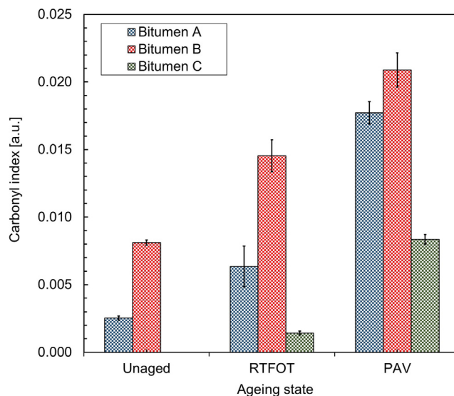
Fig. 5. Evolution of carbonyl index with ageing.
