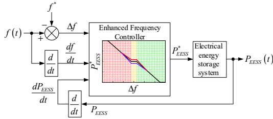
Fig. 5. EFR controller integrated with the EESS to control output power ( P_{EES} ) and ramp rate ( dP_{EES}/dt ). f^* is the nominal system frequency (50 Hz) [4].
