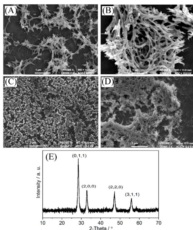
Figure 2. Electron micrographs of (A) a 10-layer PIM-EA-TB – \text{Pr}(\text{NO}_3)_3 (1:1) film after calcination, (B) a 20-layer PIM-EA-TB – \text{Pr}(\text{NO}_3)_3 (1:1) film after calcination, (C) a 10-layer PIM-1 – \text{Pr}(\text{NO}_3)_3 (1:1) film after calcination and (D) a higher resolution image of the same sample. (E) XRD analysis.
