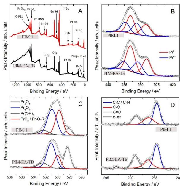
Figure 3. XPS survey spectra (A) of PIM-EA-TB and PIM-1 and core level data for (B) \text{Pr}3d_{5/2} (with red and blue curve fits for \text{Pr}^{3+} and \text{Pr}^{4+} species, respectively), (C) \text{O}1s , (D) \text{C}1s .
