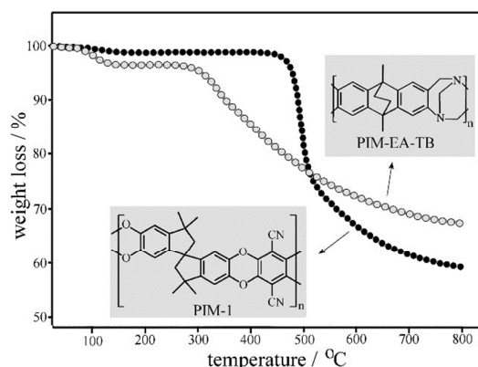
Figure 1. Thermogravimetric data and molecular structures for PIM-EA-TB and PIM-1.
