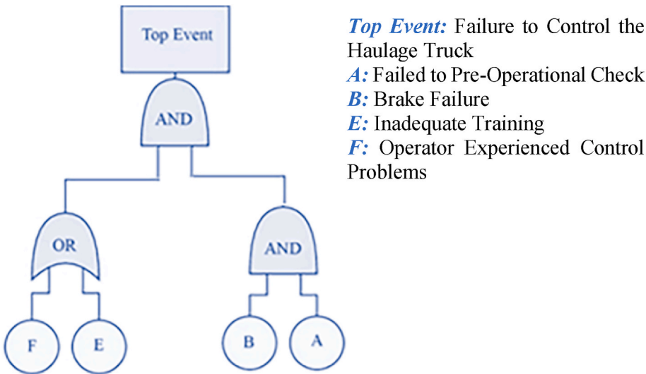
Fig. 10. An FTA structure for a scenario that the driver failed to control the haulage truck.
