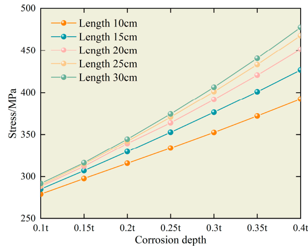
Figure 20. Stress in corroded pipeline without landslide impact.
