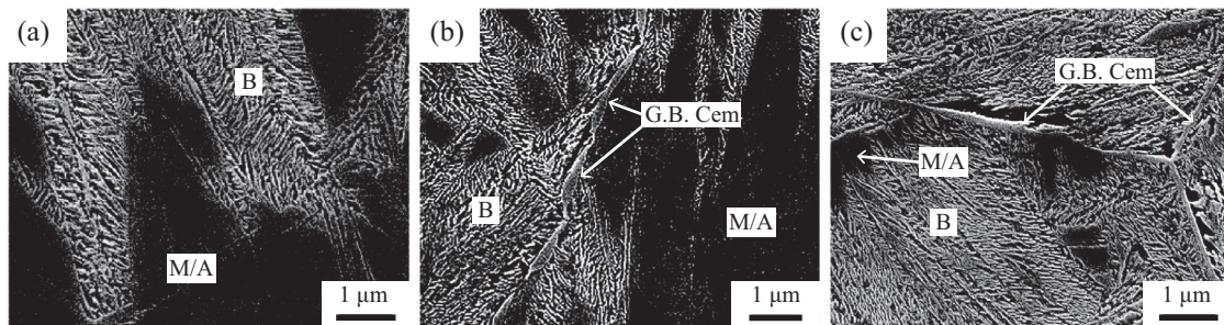
Fig. 3. SEM micrographs obtained after bainite formation treatment when it preceded by (a) no IAT (b) IAT at 500 °C for 10 min and (c) IAT at 800 °C for 10 min. Microstructure studies revealed Bainite (B), Martensite/Retained austenite (M/A) islands and grain-boundary cementite (G.B. Cem) depending on the corresponding treatment route.
