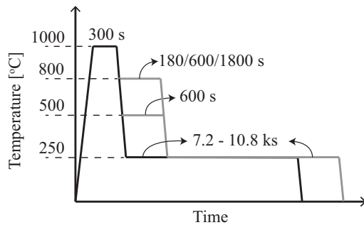
Fig. 1. Schematic of heat treatment profiles used for understanding the effect of grain-boundary cementite precipitation on bainite formation kinetics. The heating rate used during the heat treatments is 5 °C/s while the all cooling steps are carried out at −40 °C/s.
