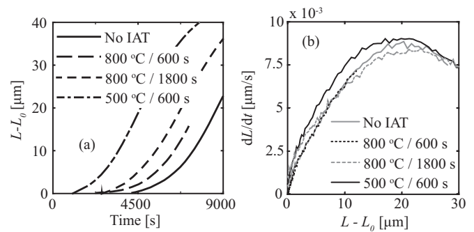
Fig. 2. (a) Bainite evolution obtained via different heat treatment routes represented in terms of change in length of the sample during isothermal holding at 250 °C (b) Rate of change of length of sample as a function of sample expansion during isothermal holding at 250 °C. No IAT refers to the heat treatment where IAT was not applied prior to bainite formation. The rest of the curves were obtained after an IAT was employed. The time and temperature of the IAT is mentioned in the legend.
