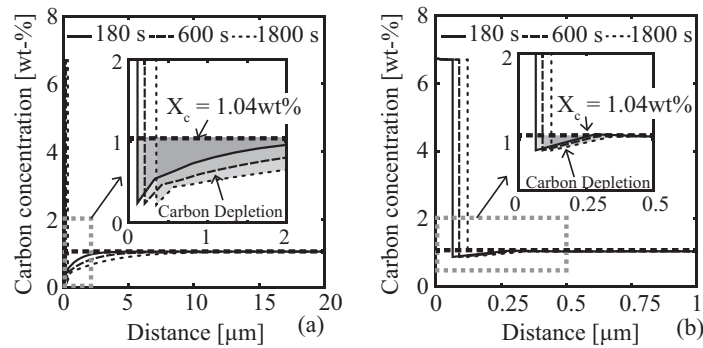
Fig. 4. Variation in carbon concentration in the vicinity of cementite/austenite interface as a result of cementite precipitation after isothermal holding at (a) 500 °C and (b) 800 °C for different times based on DICTRA calculations simulating IAT. Shaded regions indicate the carbon depleted regions. Simulations indicate moving cementite/austenite interface during the time-scale of IAT as well as a higher fraction of cementite formation during IAT at 500 °C.
