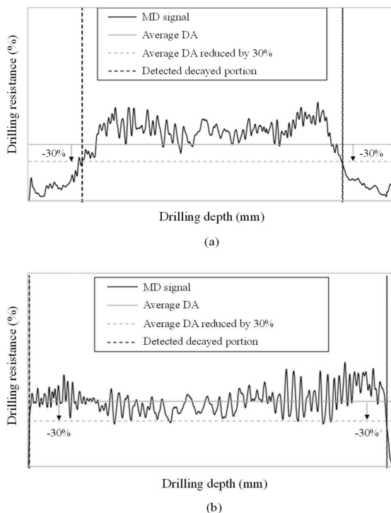
Figure 4: Procedure adopted for determining the degraded portion of the pile segments from MD signals, corresponding to low drilling amplitudes at the beginning and at the end. Examples are shown in the case of a heavily decayed pile (a) and a sound pile (b). Adapted from [3].
