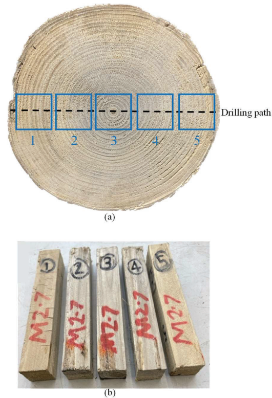
Figure 5: (a) Location of the samples taken to determine MC variations among sapwood, heartwood, and pith; (b) example of prisms retrieved from a pile segment along the drilling depth.
