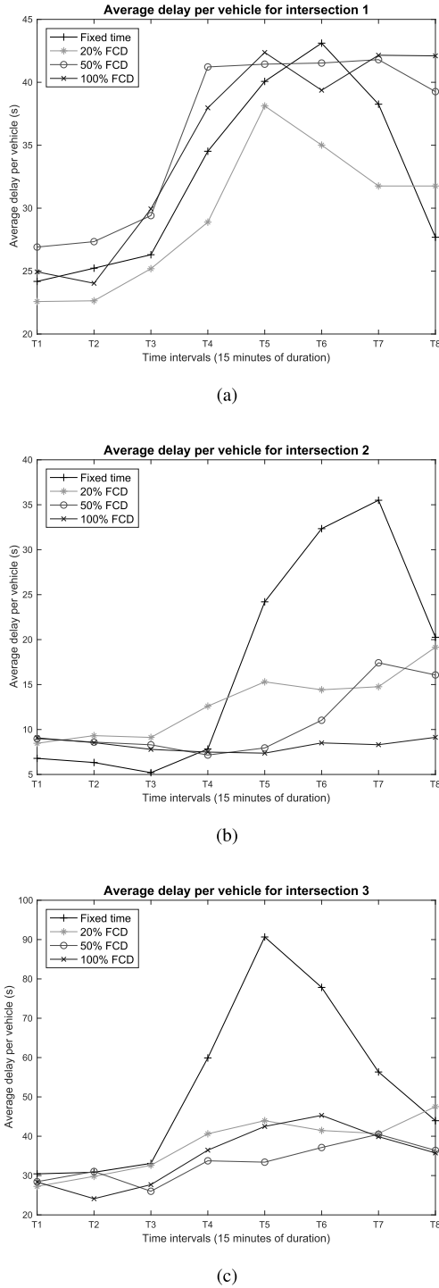
Fig. 7. (a), (b), (c) Average delay per vehicle trend over different time intervals.
