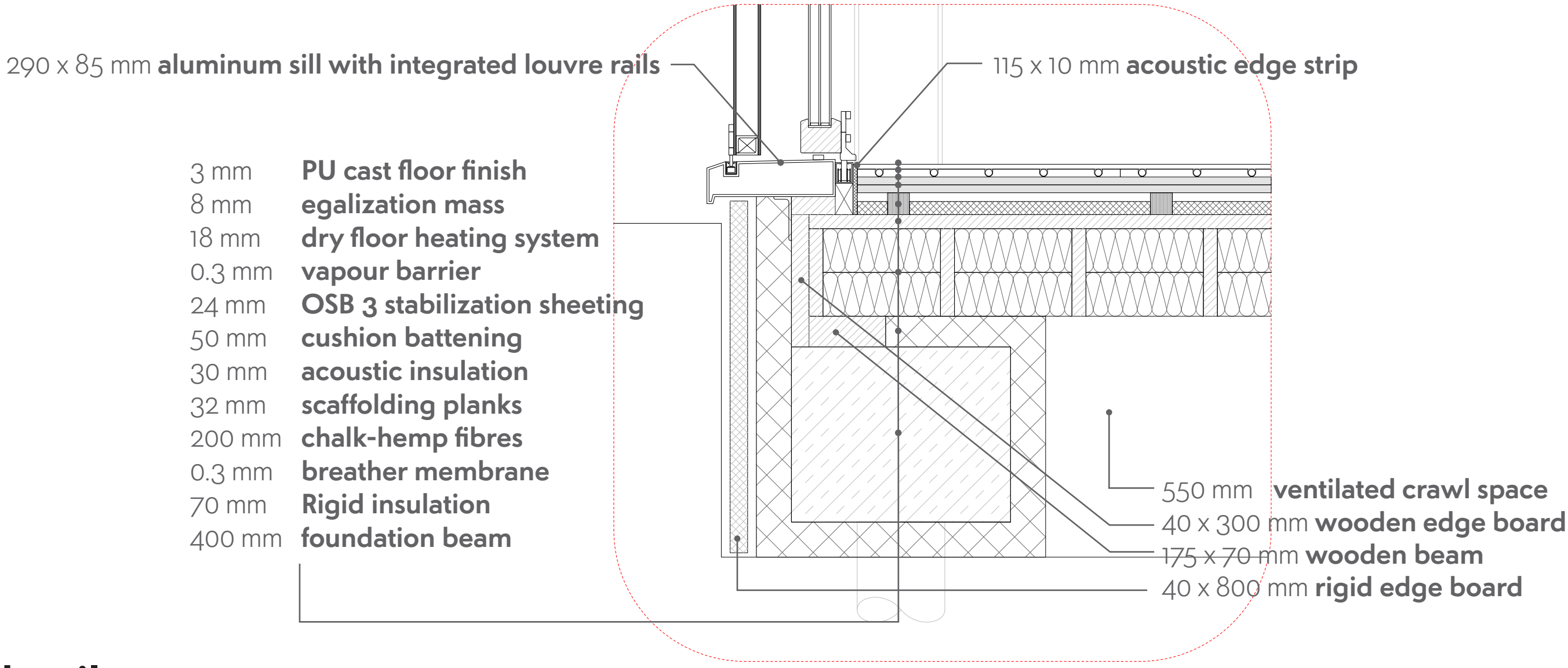
Horizontal detail 1:10
