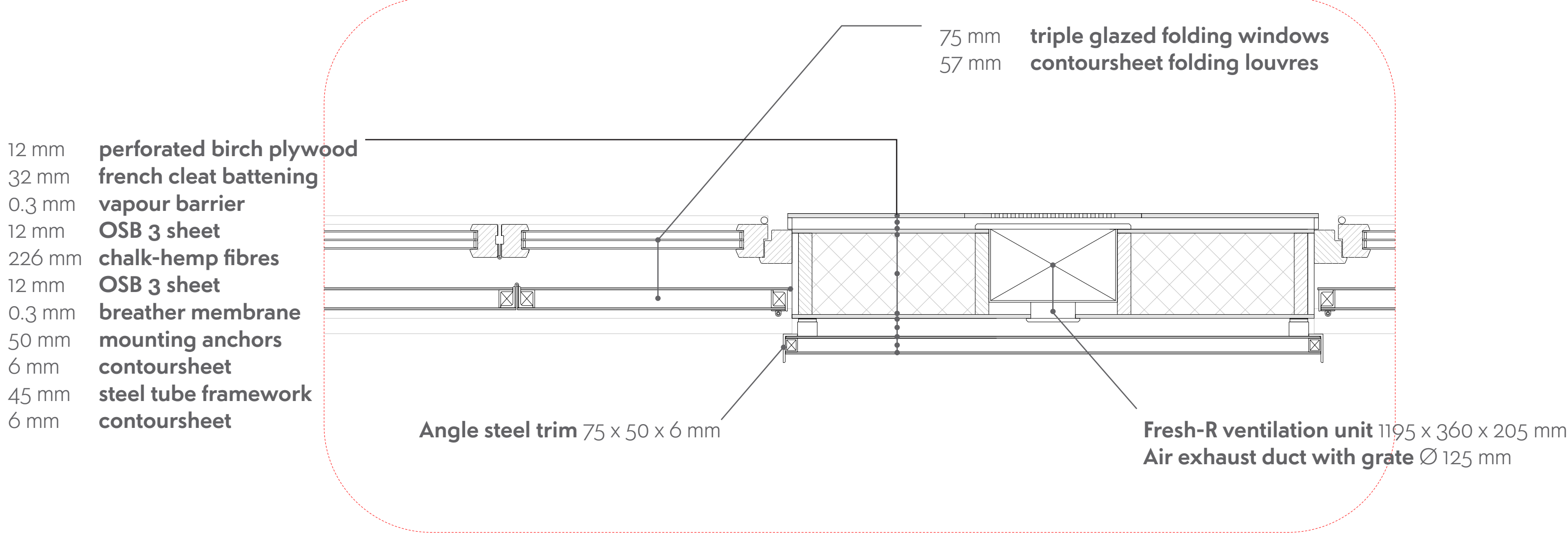
Horizontal detail 1:10
