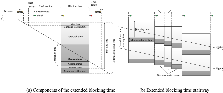
Figure 6.1: The left plot (a) shows the attributes for the extended blocking time stairway including the minimum buffer time for a three-aspect signalling system. The right plot (b) indicates a partial blocking time stairway for two successive trains including the (minimum) buffer time.
