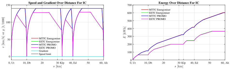
Figure 5.4: Uniform distribution scenario IC speed/gradient–distance profile (left) and energy–distance profile (right) of the MTTC and EETC driving strategies of Energymiser and PROMO.
