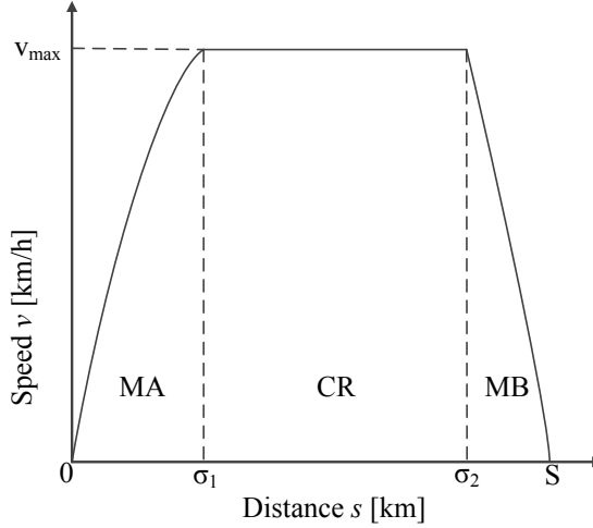
Figure 3.4: Speed profile of a basic minimum time control strategy with switching points between driving regimes at \sigma_1 and \sigma_2 for a flat track without varying speed limits (MA = maximum acceleration, CR = cruising, and MB = maximum braking).
