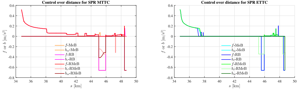
Figure 3.18: Real-life case scenario for the SPR (Zbm-Ht) with the control-distance profile for the MTTC (left) and EETC (right) driving strategies.
