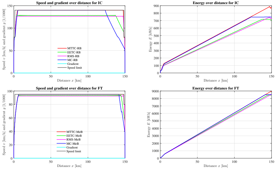
Figure 4.6: Results for scenario with a track length of 150 km for IC and FT.
