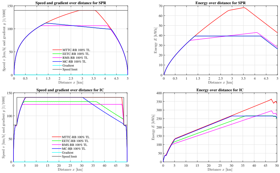
Figure 4.9: Results fully loaded scenario for SPR and IC.
