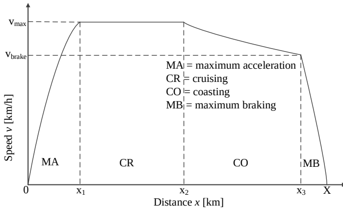
Figure 2.4: Speed profile of a basic energy-efficient driving strategy with switching points between driving regimes at x_1 , x_2 and x_3 .
