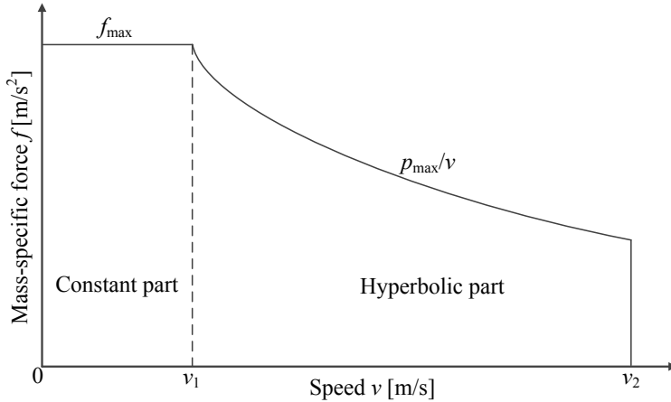
Figure 5.1: Typical specific traction-speed diagram with a constant and hyperbolic part.
