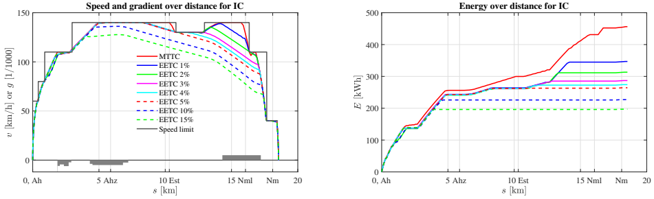
Figure 6.4: The left plot shows for the case Ah-Nm IC with varying running time supplements the speed/gradient–distance profile of the MTTC and EETC driving strategies. The right plot indicates the energy–distance profile of the MTTC and EETC driving strategies for the case Ah-Nm IC.
