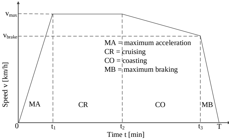
Figure 2.1: Optimal driving regimes for energy-efficient driving on flat track as function of time with switching points at t_1 , t_2 and t_3 .
