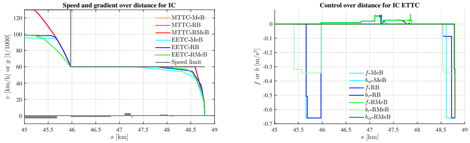
Figure 3.16: Real-life case scenario for the IC (Ut-Ht) zoomed in between 45 km and 49 km for the braking behavior of the energy-efficient driving strategies with the speed/gradient-distance profile (left) and control-distance profile (right). The grey area in the left figure indicates the gradients [\text{‰}] .
