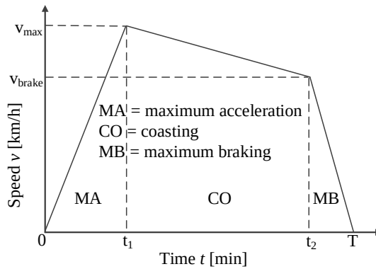
Figure 2.3: Optimal driving regimes without cruising (for metro and suburban railway systems) over time with switching points between driving regimes at t_1 and t_2 .
