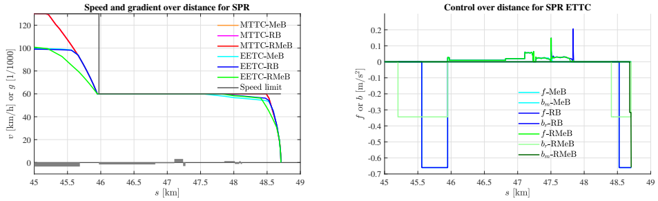
Figure 3.19: Real-life case scenario for the SPR (Zbm-Ht) zoomed in between 45 km and 49 km for the braking behavior of the energy-efficient driving strategies with the speed/gradient-distance profile (left) and control-distance profile (right). The grey area in the left figure indicates the gradients [ \% ].
