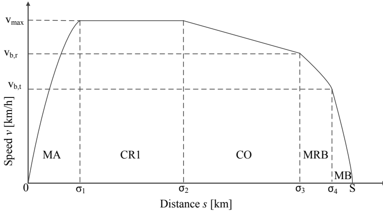
Figure 3.2: Speed profile of a basic energy-efficient driving strategy with regenerative and mechanical braking including switching points between driving regimes at \sigma_1 , \sigma_2 , \sigma_3 , and \sigma_4 for a flat track without varying speed limits and sufficient running time supplements ( v_{\max} = optimal cruising speed, v_{b,r} = speed at the start of the MRB regime, v_{b,t} = speed at the start of the MB regime, MA = maximum acceleration, CR1 = cruising by partial traction, CO = coasting, MRB = maximum regenerative braking, and MB = maximum braking).
