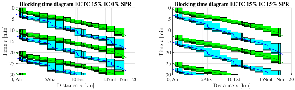
Figure 6.9: The left plot shows for the case Ah-Nm for the IC (green) and SPR (blue) compressed blocking time diagram for the EETC driving strategies with 15% running time supplements for the IC and 0% running time supplements for the SPR. The right plot indicates the IC (green) and SPR (blue) compressed blocking time diagram for the case Ah-Nm for the EETC driving strategies with 15% running time supplements for both the IC and SPR.
