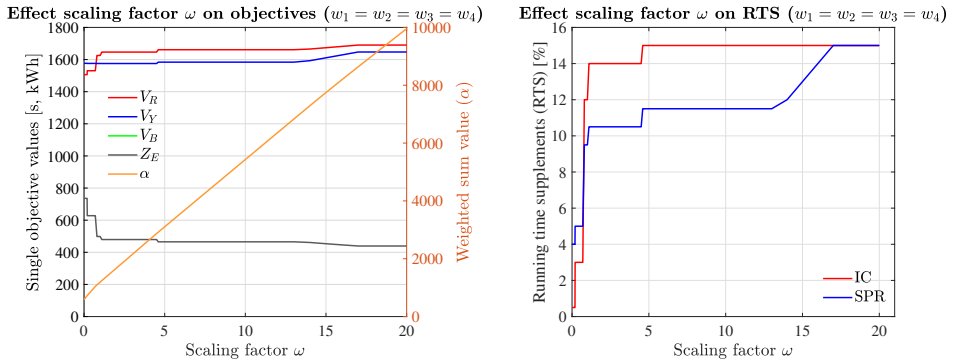
Figure 6.13: The left plot shows the sensitivity analysis by varying the scaling factor of the energy consumption \omega related to the single objectives (left y-axis) and weighted sum value (right y-axis). The right plot indicates the running time supplements (RTS) for the IC and SPR given the varying weight factor of the energy consumption \omega .
