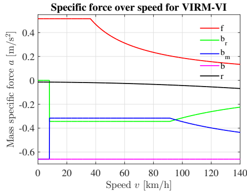
Figure 3.5: Mass-specific force-speed diagram for VIRM-VI ( f : mass-specific traction force, r : mass-specific train resistance, b_r : mass-specific regenerative braking force, and b_m : mass-specific mechanical braking force).
