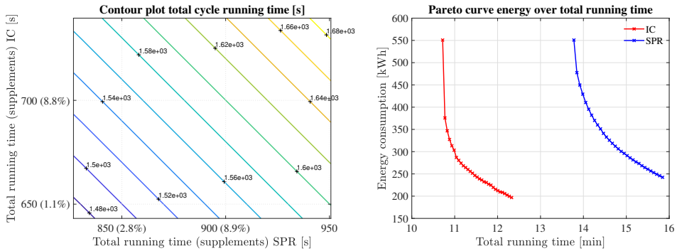
Figure 6.6: The left plot shows the contour plot for the case Ah-Nm for the total cycle running time over the total running time (supplements) for the SPR and IC. The right plot indicates the Pareto frontier curve of the energy consumption over the total running time for the IC and SPR for the case Ah-Nm.
