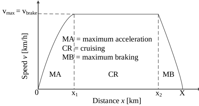
Figure 2.6: Speed profile of an energy-efficient driving strategy without coasting and with switching points between driving regimes at x_1 and x_2 .
