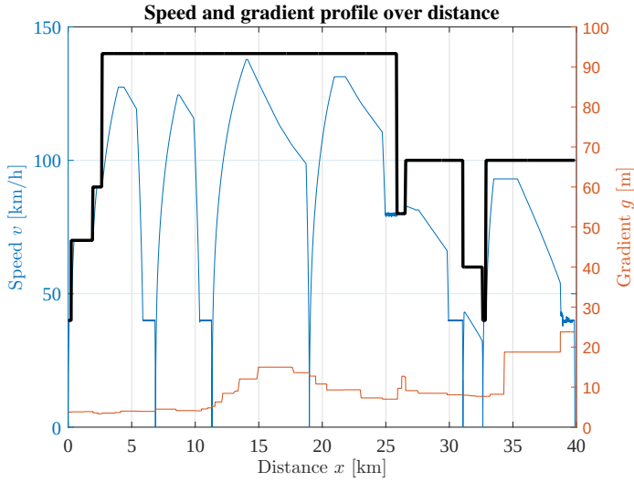
Figure 2.5: Example of an energy-efficient speed profile with varying gradients and speed limits for the line Utrecht Central-Rhenen (adapted from Scheepmaker & Goverde (2015)).
