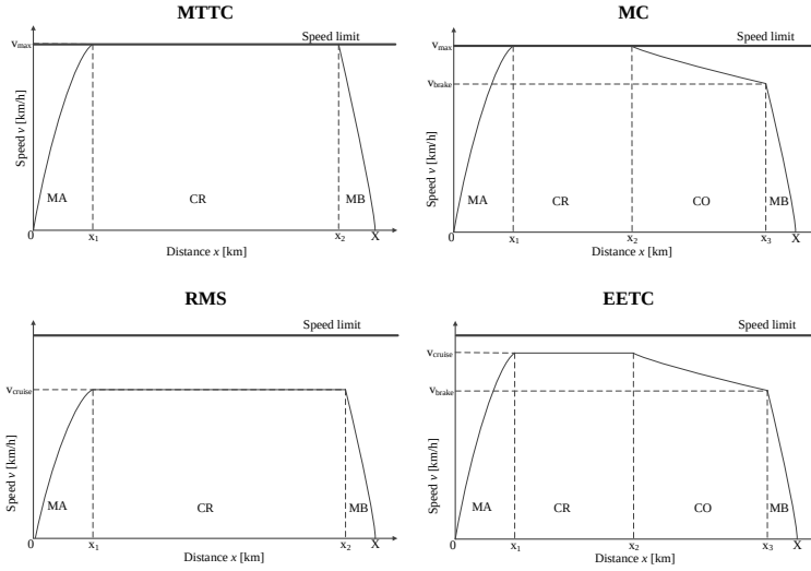
Figure 4.2: The different driving strategies: MTTC (top left), MC (top right), RMS (bottom left), and EETC (bottom right). (MA = maximum acceleration, CR = cruising, CO = coasting and MB = maximum (service) braking, and the switching points x_1 , x_2 , and x_3 between driving regimes).
