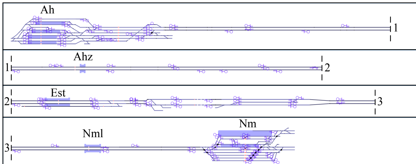
Figure 6.3: Detailed track layout of railway line Arnhem Central (Ah)–Nijmegen (Nm).
