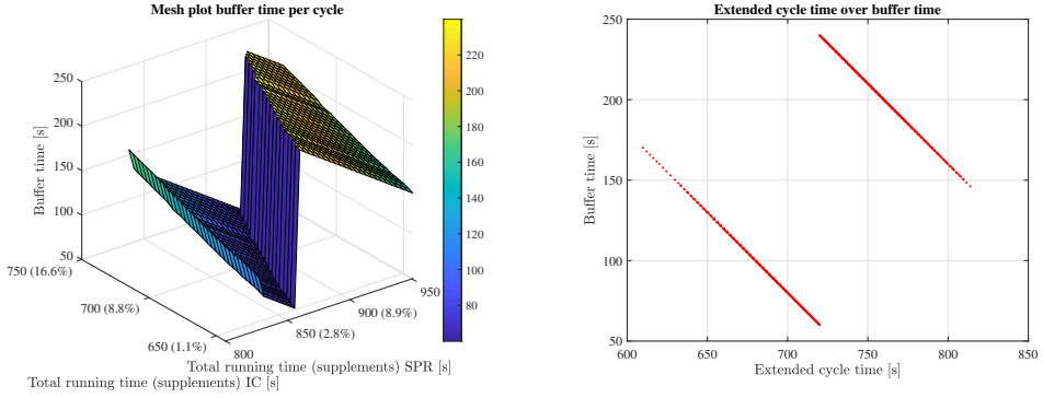
Figure 6.10: The left plot shows the mesh plot for the case Ah-Nm for the buffer time per cycle over the running time (supplements) of the SPR and IC. The right plot indicates the buffer time over extended cycle time for the case Ah-Nm.
