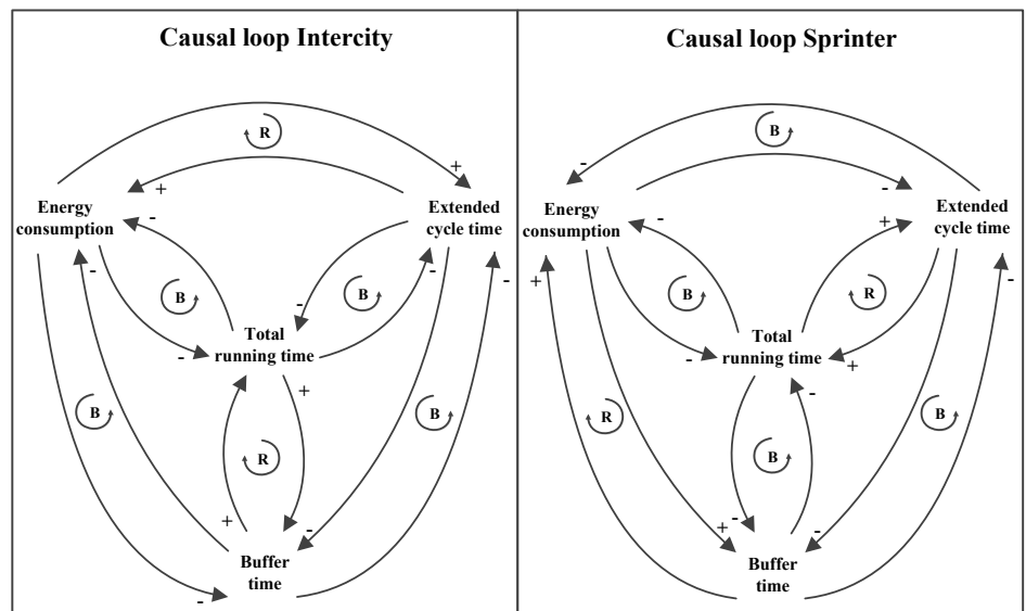
Figure 6.11: The left plot shows for the case Ah-Nm the causal loop diagram between the objectives for the IC. The right plot indicates for the case Ah-Nm the causal loop diagram between the objectives for the SPR (legend: R = Reinforcing, B = Balancing, + = objective at the end of the arrow is moving in the same direction as the objective at the beginning of the arrow, and - = objective at the end of the arrow is moving in the opposite direction as the objective at the beginning of the arrow).
