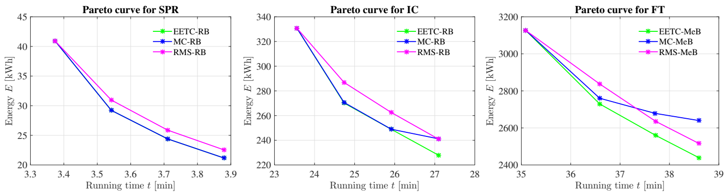
Figure 4.12: Pareto curves varying running time (left SPR, middle IC, and right FT).
