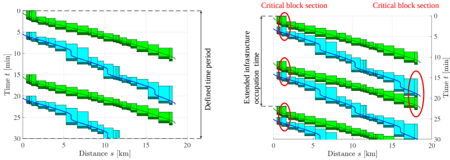
Figure 6.2: The left plot shows the timetable compression method with timetable before compression. The right plot indicates the timetable compression method with timetable after compression including the minimum buffer time and the critical blocks. Note that the darker area below the blocks indicates the minimum buffer time between trains that are included in the extended blocking times.
