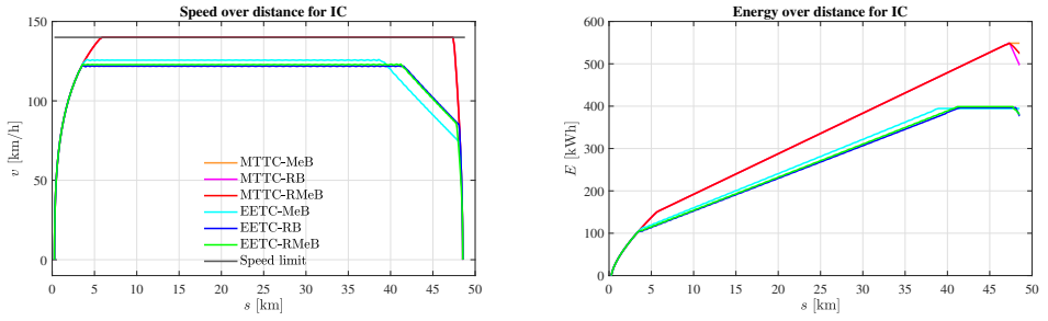
Figure 3.7: Reference scenario for the IC with the speed-distance profile (left) and energy-distance profile of the different driving strategies (right).
