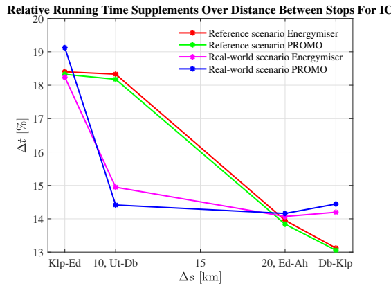
Figure 5.3: Relative running time supplements ( \Delta t ) over the distance between two stops ( \Delta s ) for the reference scenario and real-world scenario (i.e., including varying gradients and speed limits) by using the models of Energymiser and PROMO.
