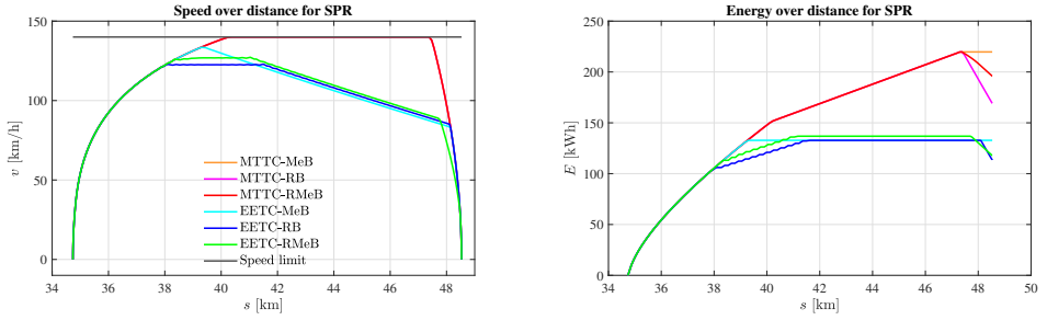
Figure 3.11: Reference scenario for the SPR with the speed-distance profile (left) and energy-distance profile of the different driving strategies (right).
