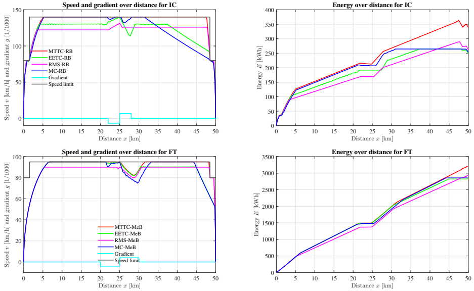
Figure 4.7: Results varying gradient scenario for IC and FT.
