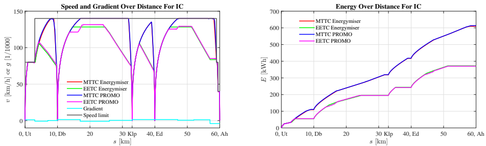
Figure 5.6: Real-world case scenario IC (Ut–Ah) speed/gradient–distance profile (left) and energy–distance profile (right) of the MTTC and EETC driving strategies of Energymiser and PROMO.
