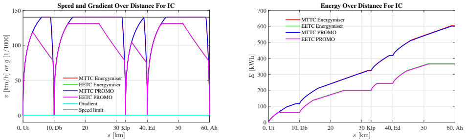
Figure 5.2: Reference scenario IC speed/gradient-distance profile (left) and energy-distance profile (right) of the MTTC and EETC driving strategies of Energymiser and PROMO.
