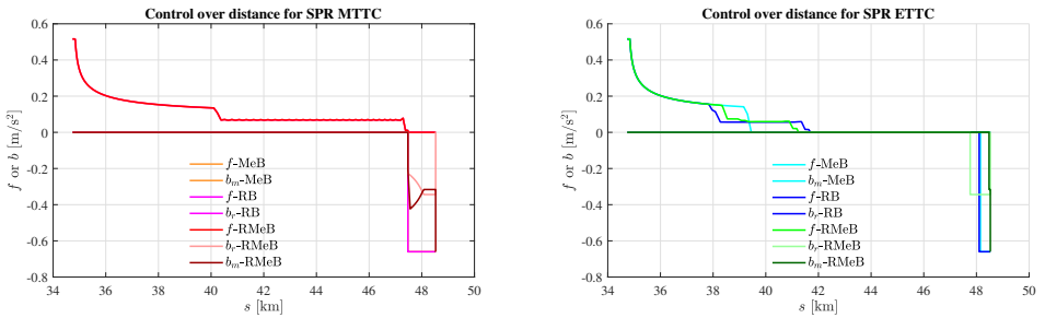
Figure 3.12: Reference scenario for the SPR with the control-distance profile for the MTT-C (left) and EETC (right) driving strategies.
