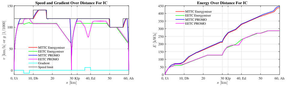
Figure 5.5: Varying gradients and speed limits scenario IC speed/gradient–distance profile (left) and energy–distance profile (right) of the MTTC and EETC driving strategies of Energymiser and PROMO.
