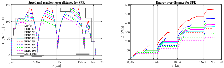
Figure 6.5: The left plot shows for the case Ah-Nm SPR with varying running time supplements the speed/gradient–distance profile of the MTTC and EETC driving strategies. The right plot indicates the energy–distance profile of the MTTC and EETC driving strategies for the case Ah-Nm SPR.
