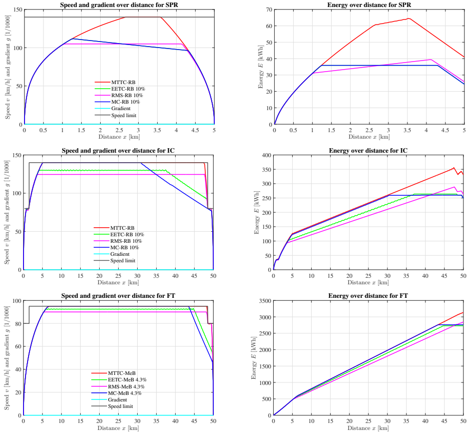
Figure 4.5: Results reference scenario. Note that for SPR the driving strategy EETC is identical to MC and, therefore, is not visible in this figure.
