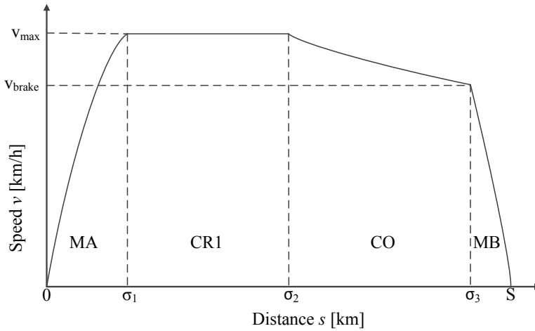
Figure 3.3: Speed profile of a basic energy-efficient driving strategy with regenerative or mechanical braking only including switching points between driving regimes at \sigma_1 , \sigma_2 and \sigma_3 for a flat track without varying speed limits and sufficient running time supplements (MA = maximum acceleration, CR1 = cruising by partial traction, CO = coasting, and MB = maximum braking).
