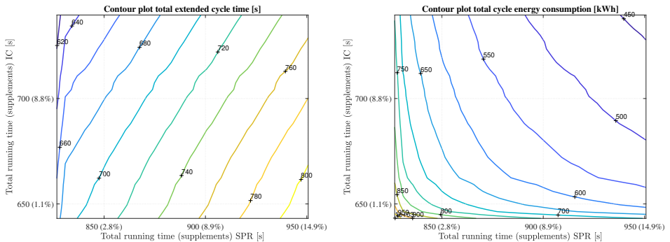
Figure 6.8: The left plot shows the contour plot for the case Ah-Nm for the extended cycle time over the total running time (supplements) for the SPR and IC. The right plot indicates the contour plot for the total total cycle energy consumption over the the total running time (supplements) for the SPR and IC for the case Ah-Nm.
