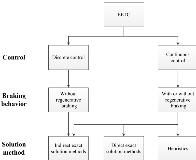
Figure 2.2: Framework of EETC.
