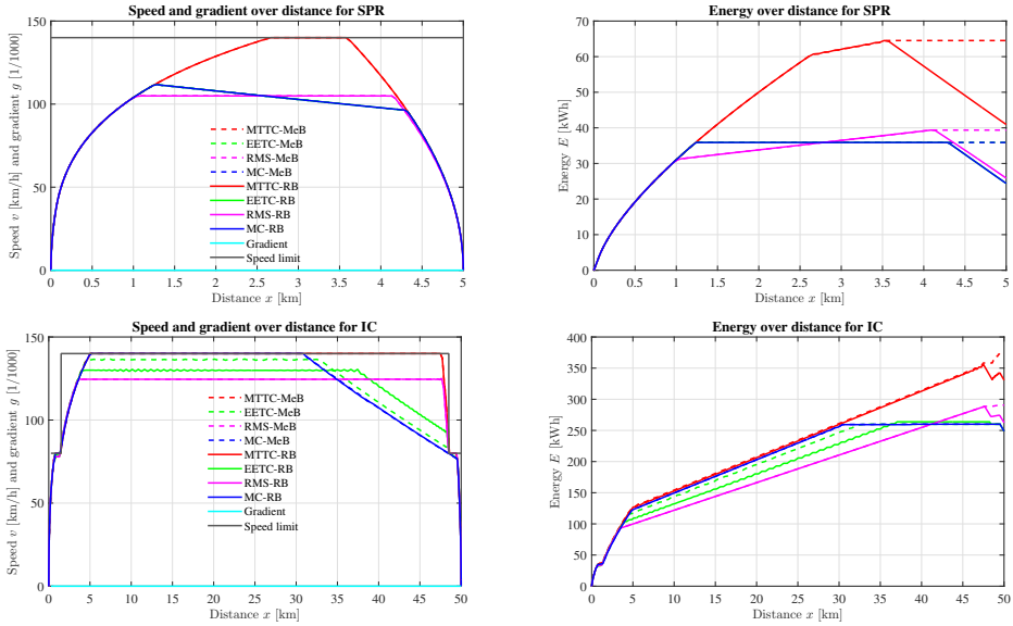
Figure 4.10: Results mechanical versus regenerative braking scenario for SPR and IC.
