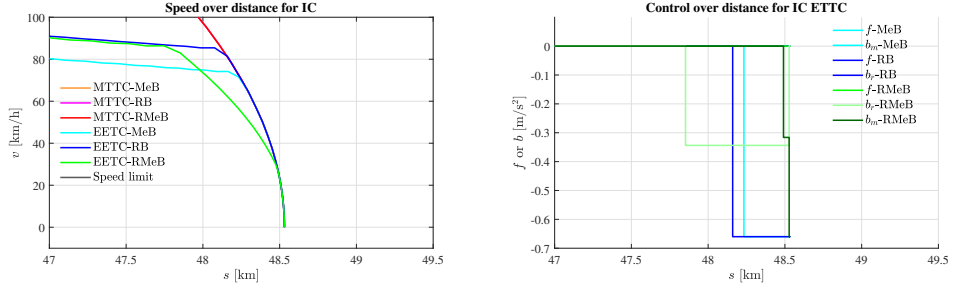
Figure 3.9: Reference scenario for the IC zoomed in for the braking behavior of the energy-efficient driving strategies with the speed-distance profile (left) and control-distance profile (right).
