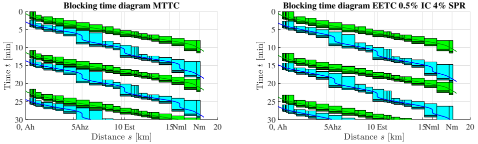
Figure 6.7: The left plot shows for the case Ah-Nm for the IC (green) and SPR (blue) compressed blocking time diagram of the MTTC driving strategies. The right plot indicates for the IC (green) and SPR (blue) compressed blocking time diagram EETC driving strategies for the case Ah-Nm. The EETC driving strategy has 0.5% running time supplements for the IC and 4% running time supplements for the SPR. The dark green and dark blue blocks are the minimum buffer time of 30 s.
