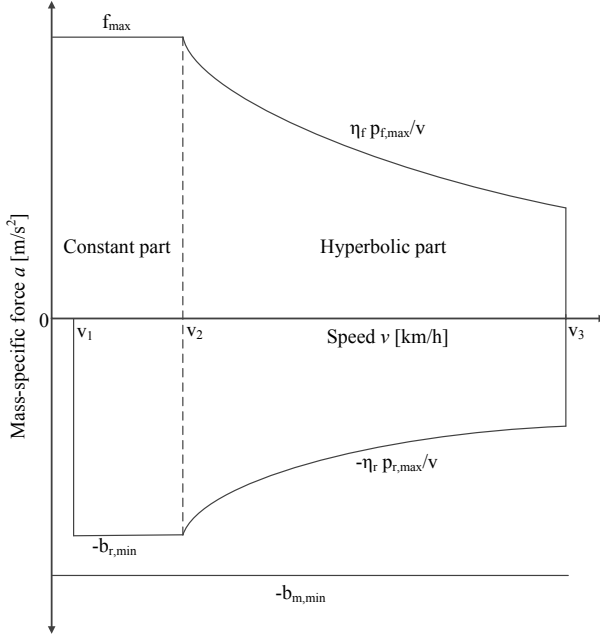
Figure 3.1: Typical mass-specific traction-speed ( f ) and mass-specific regenerative braking-speed ( b_r ) diagram with a constant and hyperbolic part, and a constant mass-specific mechanical braking force b_m . The mass-specific regenerative braking force is zero below speed v_1 .
