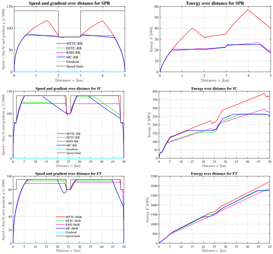
Figure 4.11: Results speed restriction scenario.
