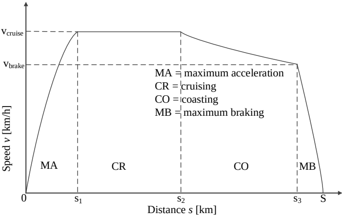
Figure 1.3: Speed profile of a basic energy-efficient driving strategy with switching points between driving regimes at s_1 , s_2 and s_3 for a flat track with sufficient running time supplements.
