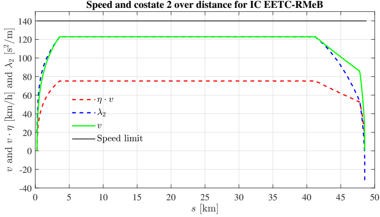
Figure 3.6: Validation of the reference scenario for the IC with the EETC-RMeB driving strategy by using the speed/costate \lambda_2 -distance profile.
