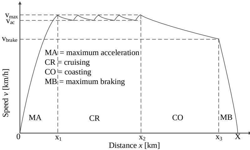
Figure 2.7: Speed profile of an energy-efficient driving strategy with discrete control (throttle settings) with switching points between driving regimes at x_1 , x_2 and x_3 (the cruising phase consists of different phases of acceleration and coasting).
