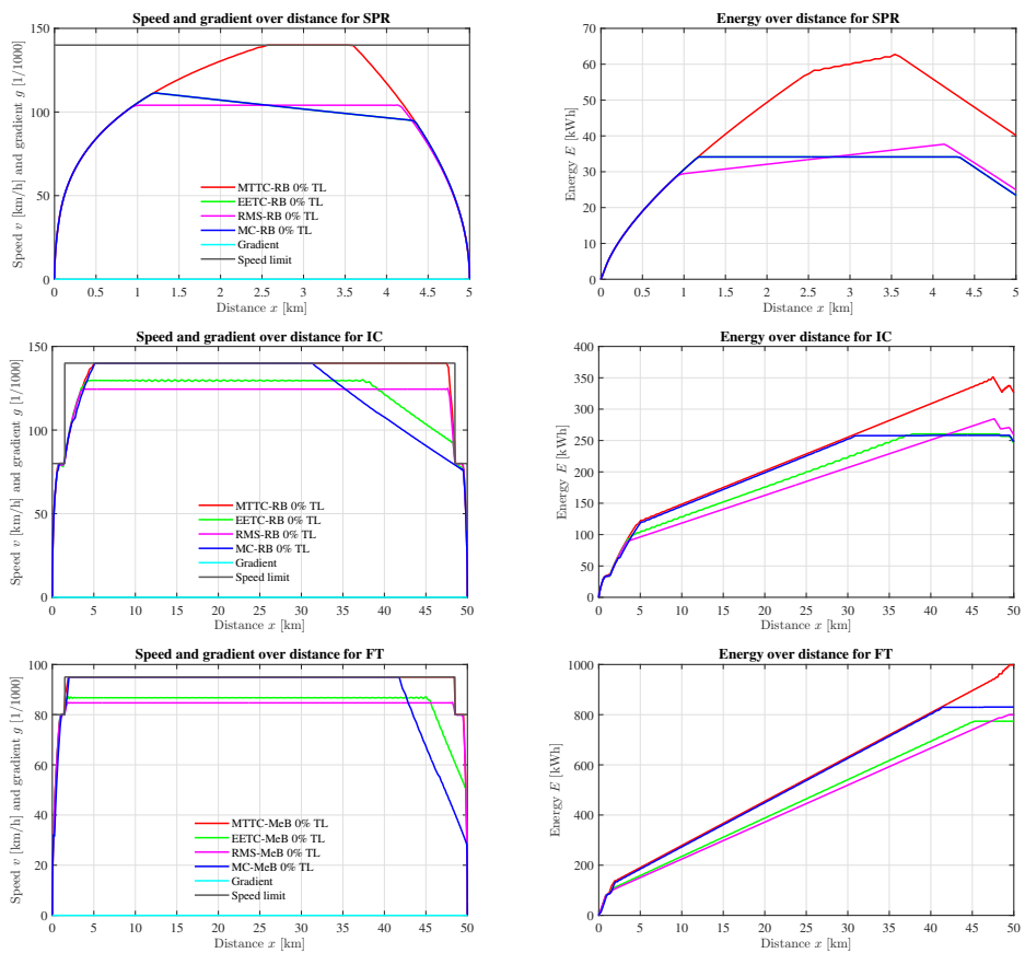
Figure 4.8: Results zero load scenario.
