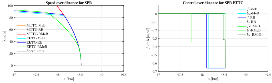
Figure 3.13: Reference scenario for the SPR zoomed in for braking behavior of the energy-efficient driving strategies with the speed-distance profile (left) and control-distance profile (right).
