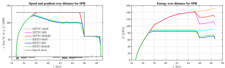
Figure 3.17: Real-life case scenario for the SPR (Zbm-Ht) with the speed/gradient-distance profile (left) and energy-distance profile of the different driving strategies (right). The grey area in the left figure indicates the gradients [%].
