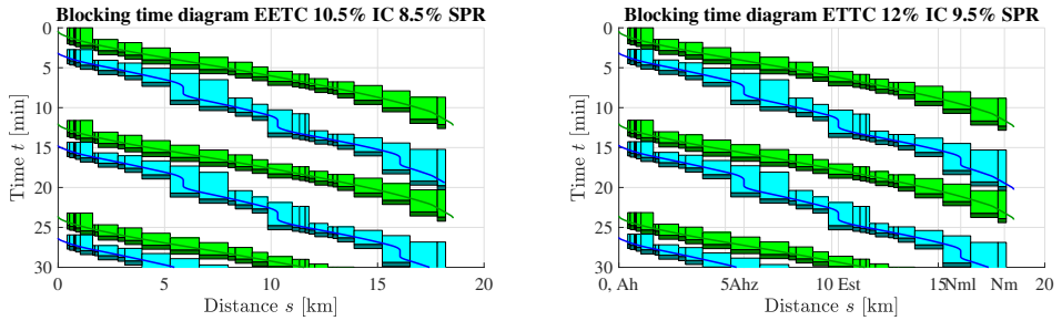
Figure 6.14: The left plot shows for the case Ah-Nm for the IC (green) and SPR (blue) compressed blocking time diagram for the EETC driving strategies with 10.5% running time supplements for the IC and 8.5% running time supplements for the SPR. The right plot indicates the IC (green) and SPR (blue) compressed blocking time diagram for the case Ah-Nm for the EETC driving strategies with 12% running time supplements for the IC and 9.5% running time supplements for the SPR.
