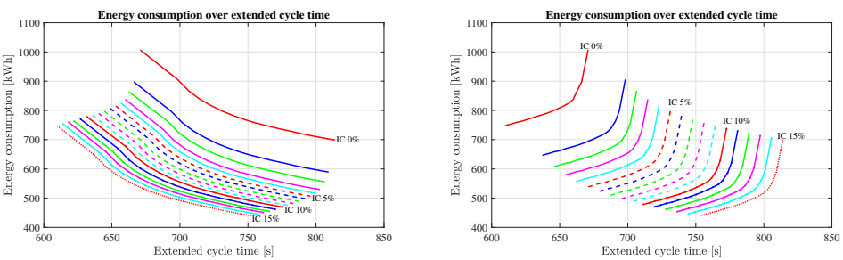
Figure 6.12: The left plot shows the energy consumption over the extended cycle time for the case Ah-Nm for fixed running time supplements of the IC and varying running time supplements for the SPR. The right plot indicates the energy consumption over the extended cycle time for fixed running time supplements of the SPR and varying running time supplements for the IC for the case Ah-Nm.
