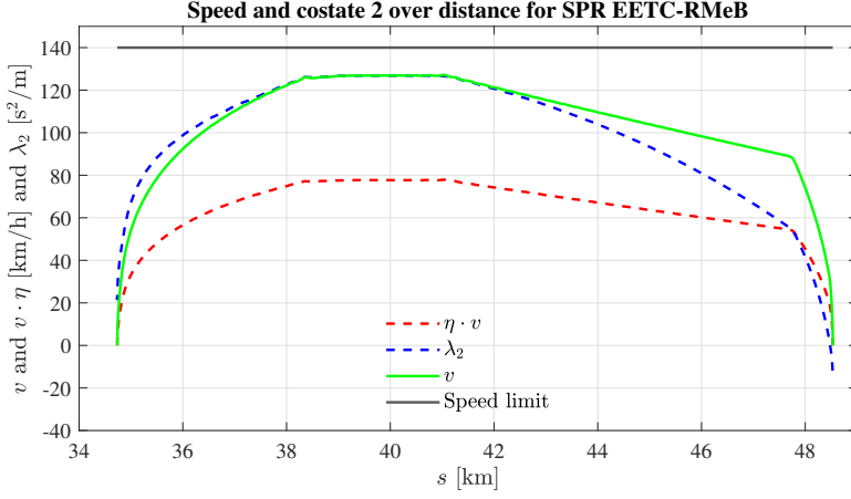
Figure 3.10: Validation of the reference scenario for the SPR with the EETC-RMeB driving strategy by using the speed/costate \lambda_2 -distance profile.
