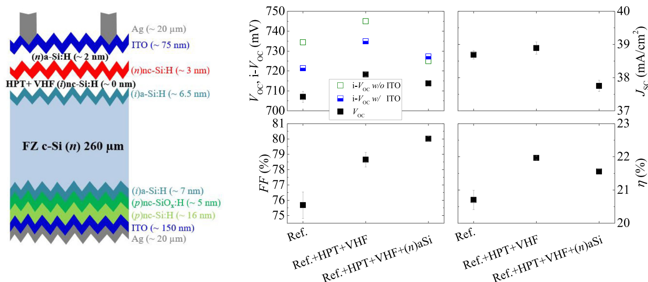
FIGURE 8 The schematic sketches and external parameters of rear junction FBC-SHJ cells featuring 3-nm-thick (n)nc-Si:H as (n)-type contact as function of HPT + VHF (i)nc-Si:H and (n)a-Si:H capping layer treatments. Solar cells without any treatment are denoted as the reference (Ref.). The VHF (i)nc-Si:H is abbreviated as VHF. Note that we have not observed any detectable layer growth or etching by SE after 6 minutes of VHF (i)nc-Si:H deposition. The results represent averaged parameters with four solar cells (3.92 cm 2 ) and the error bars represent the standard deviations [Colour figure can be viewed at wileyonlinelibrary.com ]
