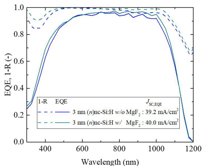
FIGURE 10 The EQE and 1-R spectra of rear junction FBC-SHJ cell featuring 3-nm-thick (n)nc-Si:H with and without \text{MgF}_2 for forming DLARC with ITO [Colour figure can be viewed at wileyonlinelibrary.com ]
