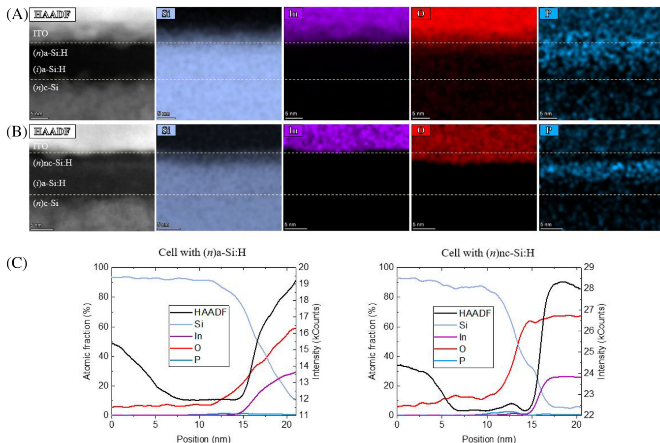
FIGURE 7 The scanning TEM (STEM) high-angle annular dark-field (HAADF) images combined with chemical compositional mapping measured by EDX of solar cells with (A) ~4-nm-thick (n)a-Si:H, and (B) ~3-nm-thick (n)nc-Si:H (n)-contacts. The white dashed lines are guides to the eyes for distinguishing (n)c-Si/(i)a-Si:H and (n)-contact/ITO interfaces. Note that the P signal detected outside P-rich zones is an artifact, just as the O signal in the c-Si substrate. Part (C) presents the atomic fractions (intensity) of different elements (HAADF) for EDX mapping results that are shown in Parts (A) and (B). The “O-nm” position lies inside the (n)c-Si wafer and it is close to the (n)c-Si/(i)a-Si:H interface [Colour figure can be viewed at wileyonlinelibrary.com ]
