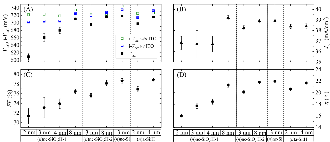
FIGURE 4 The J-V characteristics of rear junction FBC-SHJ solar cells with various (n)-type contacts: (A) i-V_{\text{OC}} and V_{\text{OC}} , (B) J_{\text{SC}} , (C) FF, and (D) \eta . The results represent averaged parameters of four solar cells (3.92 cm 2 ) and the error bars represent the standard deviations [Colour figure can be viewed at wileyonlinelibrary.com ]
