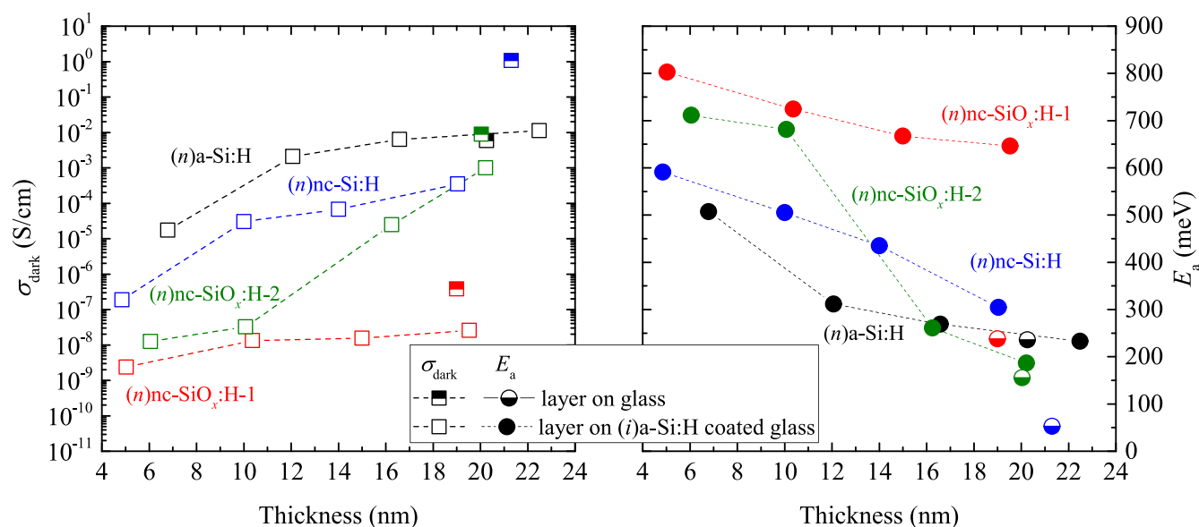
FIGURE 2 The \sigma_{\text{dark}} (left) and E_a (right) of (n)nc-SiO x :H, (n)nc-Si:H and (n)a-Si:H layers as function of layer thickness and of the different substrates [Colour figure can be viewed at wileyonlinelibrary.com ]
