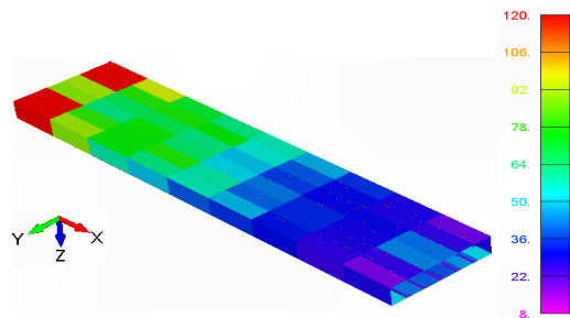
Figure 3. Optimized ply count.
