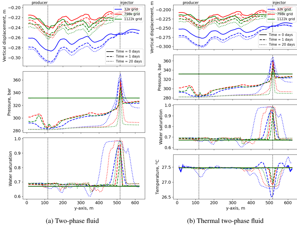
Figure 6: Solution profiles for two-phase (a) and thermal two-phase (b) fluids plotted over the longest centerline at the top of the reservoir (white line in the top-left of Fig. 4). The results are displayed for three different grid resolutions and at three time steps.
