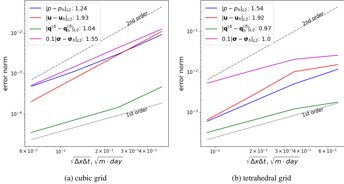
Figure 2: The L2 error norm against space-time resolution obtained with cubic (a) and tetrahedral (a) grids.
