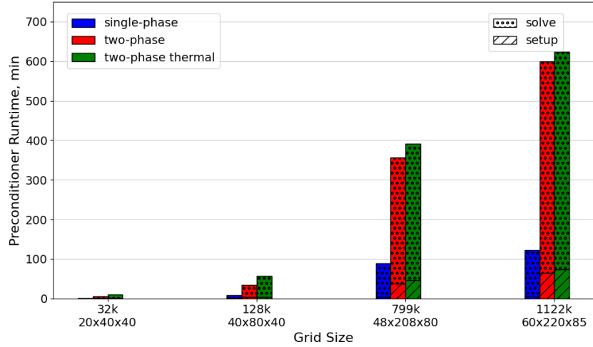
Figure 8: Cumulative runtime of the block-partitioned preconditioner to achieve convergent solutions in 20 timesteps. Timings of setup and solve calls are provided.
