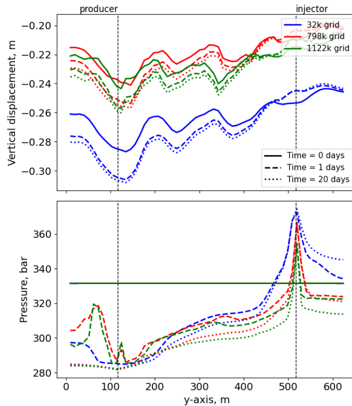
Figure 5: Solution profiles for single-phase fluid plotted over the longest centerline at the top of the reservoir (white line in the top-left of Fig. 4). The results are displayed for three different grid resolutions and at three time steps.
