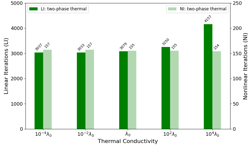
Figure 9: Sensitivity of linear (left axis) and nonlinear (right axis) iterations to the effective thermal conductivity. Calculations are performed using 24 \times 104 \times 40 grid with thermal two-phase fluid physics.
