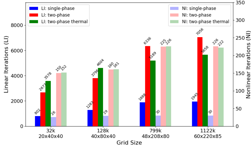
Figure 7: Scalability study of the block-partitioned preconditioner. The cumulative number of linear (left axis) and nonlinear (right axis) iterations required to achieve convergent solutions in 20 timesteps is plotted against multiple grid resolutions.
