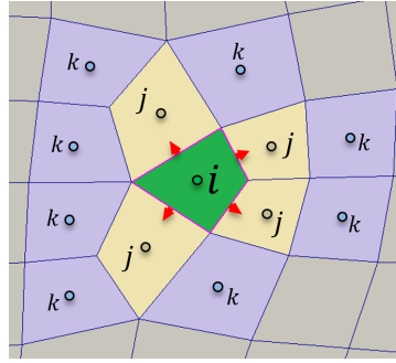
Figure 1: Cells that contribute to the approximation of fluxes over the interfaces of cell i . Index j denotes the nearest neighbors of cell i . Index k denotes farther neighbors that contribute to the gradients reconstructed in cells j .
