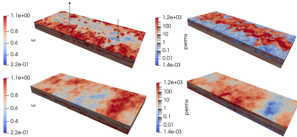
Figure 4: Young modulus (in tens of GPa) and lateral permeability (in mD) fields shown from the top (top row) and from the bottom (bottom row) of reservoir. Young's modulus is calculated as a linear function of porosity.
