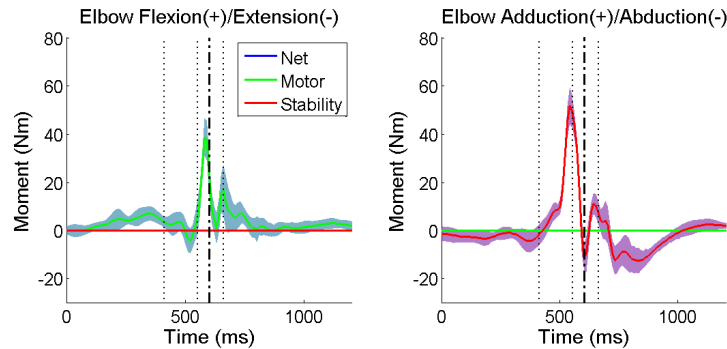
Fig3: Elbow Moments (mean \pm 1standard deviation)
