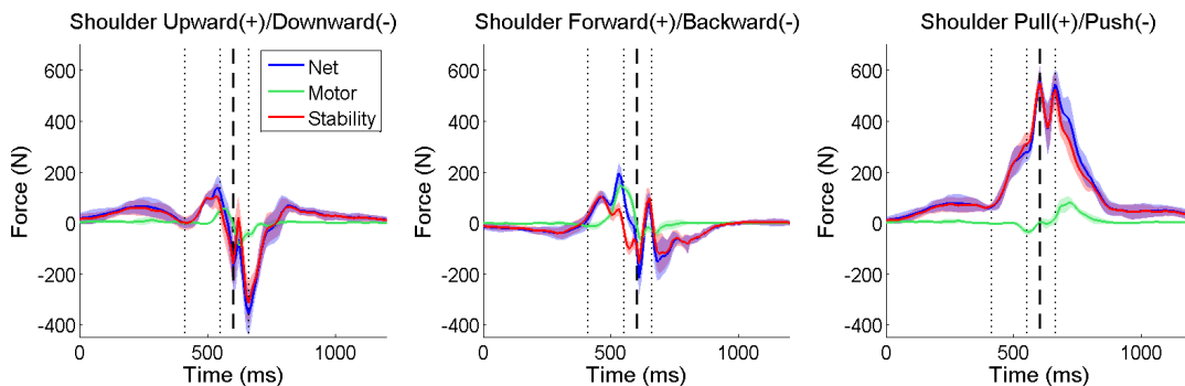
Fig5: Shoulder Force (mean \pm 1standard deviation)
