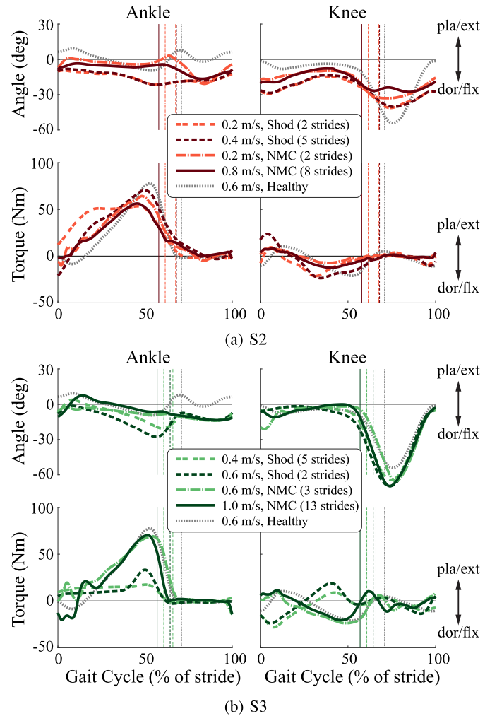
Fig. 7. Mean joint angles and torques for the right ankle and right knee for S2 and S3 as a function of stride. Walking conditions include shod (dashed or double-dashed) and NMC (solid or solid-dotted) with two different speeds (fast: dark, slow: light). Data from healthy persons (dotted) are included for comparison. Heel-strike at 0%; vertical lines indicate toe-off. Legend indicates the number of strides over which the mean was taken.
