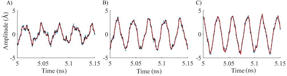
Figure 8: Time response of the center of the graphene membrane excited with different initial velocities of A) 0.1 \text{ \AA/ps} , B) 0.5 \text{ \AA/ps} , and C) 1 \text{ \AA/ps} obtained from MD (blue dots) and approximation obtained from POD with adopting 1 mode (red line) and 10 modes (black line) in a time range of 5–5.15 ns.
