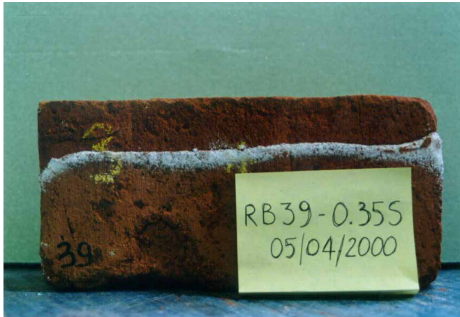
FIGS. 4.12/4.13 Salt accumulation beneath the layer treated with a water repellent (left) and subsequent spalling of the treated part (right) during a laboratory test / Photos: B. Lubelli
