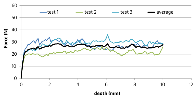
FIG. 4.22 DRMS measurements on sound Lede stone
