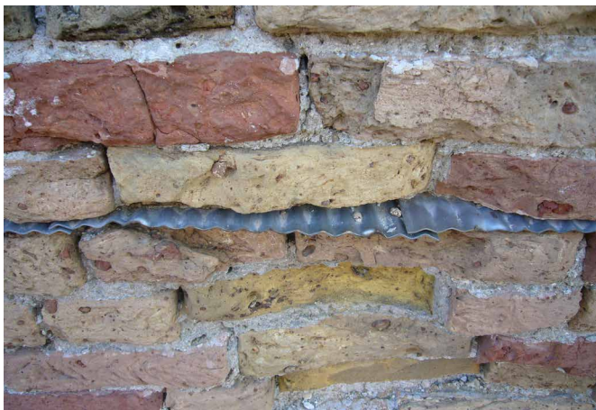
FIG. 3.4 Mechanical interruption of the wall by the use undulated steel sheets, Venice, Italy / Photo: R. van Hees
