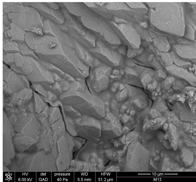
FIG. 4.9 Scanning Electron Microscopy (SEM) image showing shrinkage cracks in TEOS layer deposited in Euville limestone / Photo: TNO
