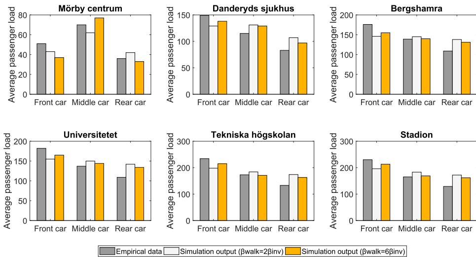
Figure 4. Average car passenger load of the simulation output for different walking time valuations and empirical data.
