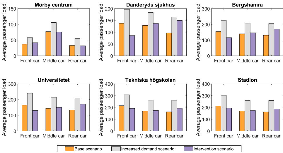
Figure 8. Average car passenger load for base, increased demand and intervention scenarios.
