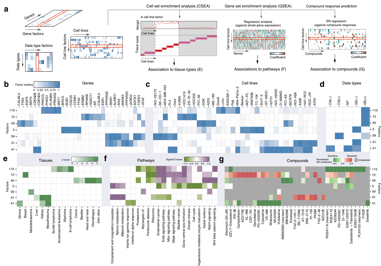
Fig. 2 Interpretation of factors obtained from WON-PARAFAC. a Assessment of tissue types enrichment; gene set enrichment and association to drug responses for cell-factors. b–d ( b ) Gene factor (gene-factor) matrix, c cell line factor (cell-factor) matrix, and d data type factor (DT-factor) matrix visualized in heatmaps, for the selected factors and their top associated genes, cell lines, and data types, respectively. Factor loading is indicated by color gradient, which is the strength of the association. e–g Associations between the selected factors and tissue types ( e ), enriched pathways ( f ), and compounds ( g ) in heatmaps where their color gradient represents the significance of association in Z-scores, signed Z-scores, and coefficients from EN, respectively. The sign in Z-score indicates up or down-regulation of pathways, and sign in EN coefficients indicates sensitivity (negative) or resistance (positive) to compounds
