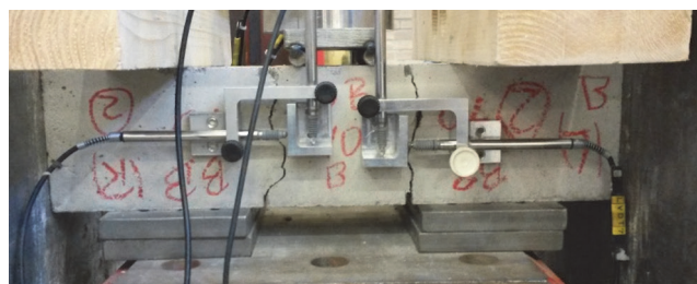
Figure 5. Experimental setup
