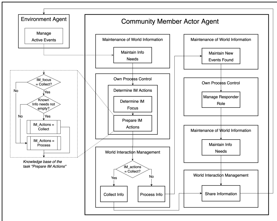
Figure 5.5: Developing a Model Narrative: narrative for the community member actor agent developed based on the model conceptualization, the specialization of the task control knowledge, and on the instantiation of the knowledge bases included in the generic model GAM. In the figure, the task control knowledge is represented by the order of execution of the tasks shown by the full arrows. An example of a knowledge base is also illustrated for the task "prepare IM Actions" through dashed lines.
