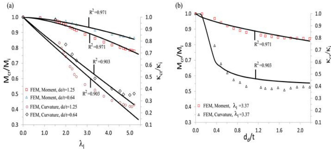
Fig. 17. Prediction of dented metallic pipes with the changing of dent parameters: (a) variation of normalized dent length ( \lambda_l = l_d / \sqrt{Rt} ); (b) variation of normalized dent depth ( d_d/t ).
