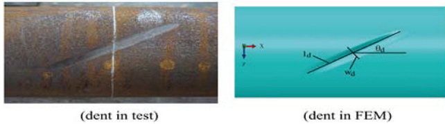
Fig. 2. The schema of dent damage on both test specimen and numerical model ( \theta_d = 45^\circ , l_d : dent length, w_d : dent width).
