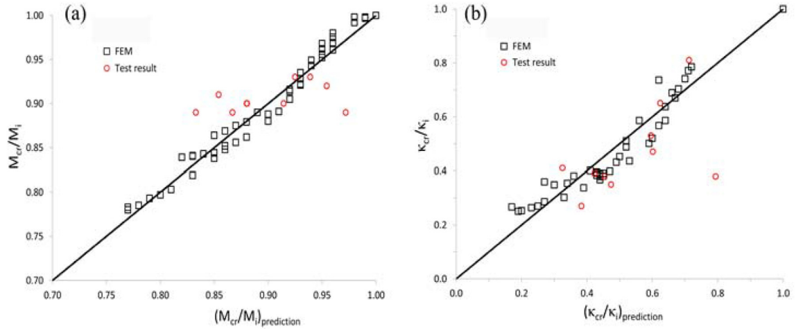
Fig. 16. Comparison between prediction of proposed equations and both experimental and numerical results: (a) normalized residual ultimate moment ( M_{cr}/M_i ); (b) normalized critical curvature ( \kappa_{cr}/\kappa_i ).
