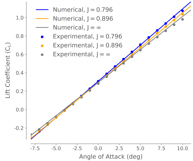
Fig. 5 Numerical and experimental [7] results of the PROWIM setup
