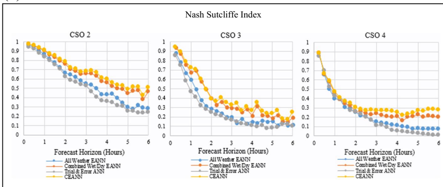
Fig. 1 a Nash-Sutcliffe Index for Case Study Sites 2, 3 & 4, and b Comparison of model performance for different ANN models for CSO site 1
