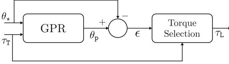
Fig. 4. Block diagram of the learning part: the inputs to the Gaussian process regressor are \theta_\star and \tau_T , while the output is the predicted bending angle \theta_p .
