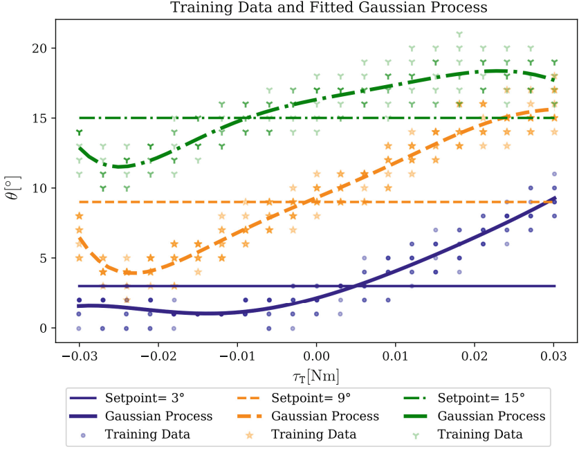
Fig. 8. A snippet of the training data. The resulting bending angle \theta for varying \tau_T . For readability, only three different desired angles \theta_\star are shown.
