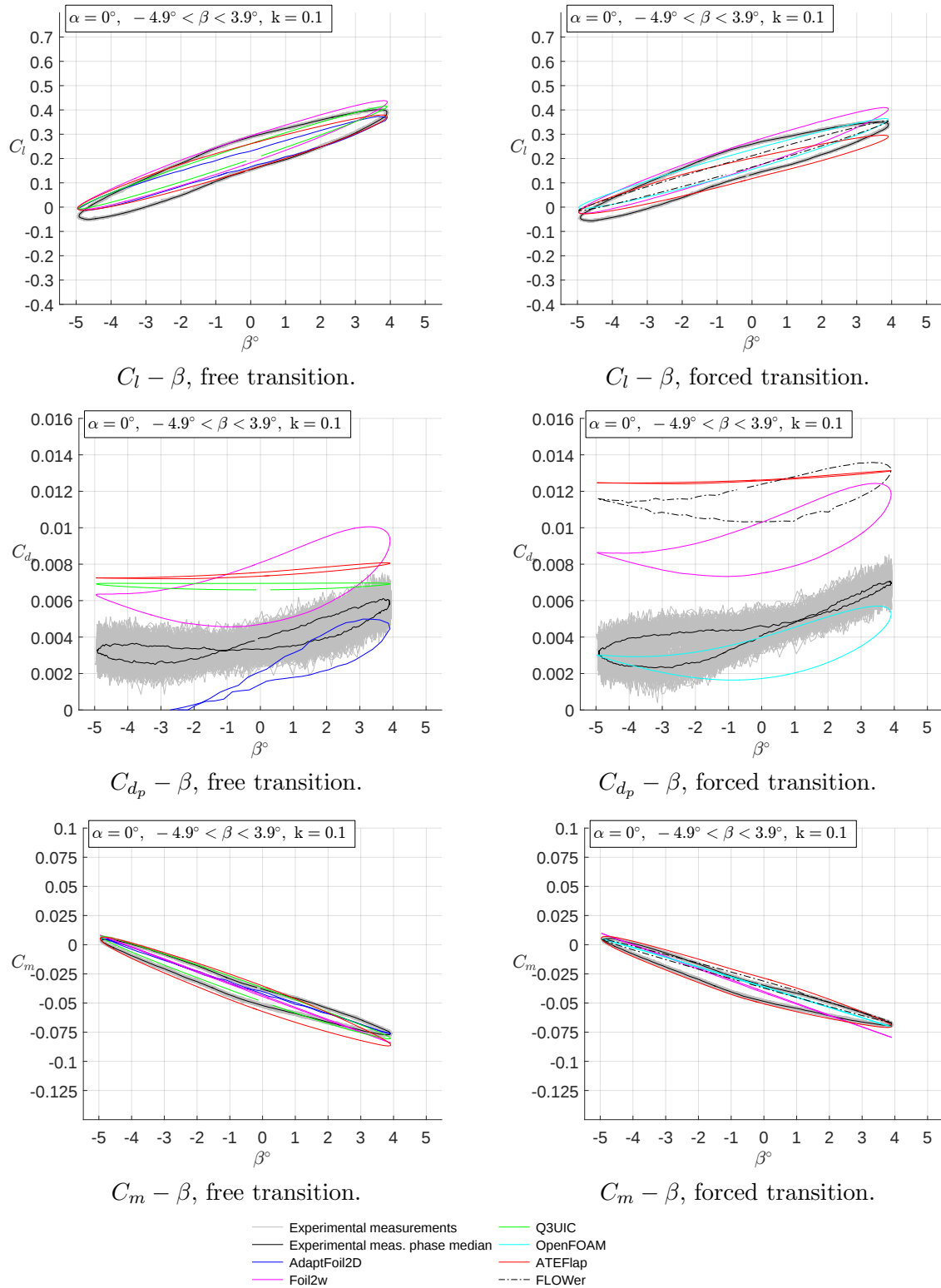
Figure 4. Validation of the numerical simulations with the unsteady experimental polars of the DU95W180 airfoil for varying flap angle and fixed angle of attack ( C_l - \beta , C_d - \beta , C_m - \beta ) at Re \approx 1.0 \cdot 10^6 , with free and forced transition, for \alpha = 0^\circ , -4.9^\circ < \beta < 3.9^\circ , k = 0.1 (cases UNST5 and UNST6).
