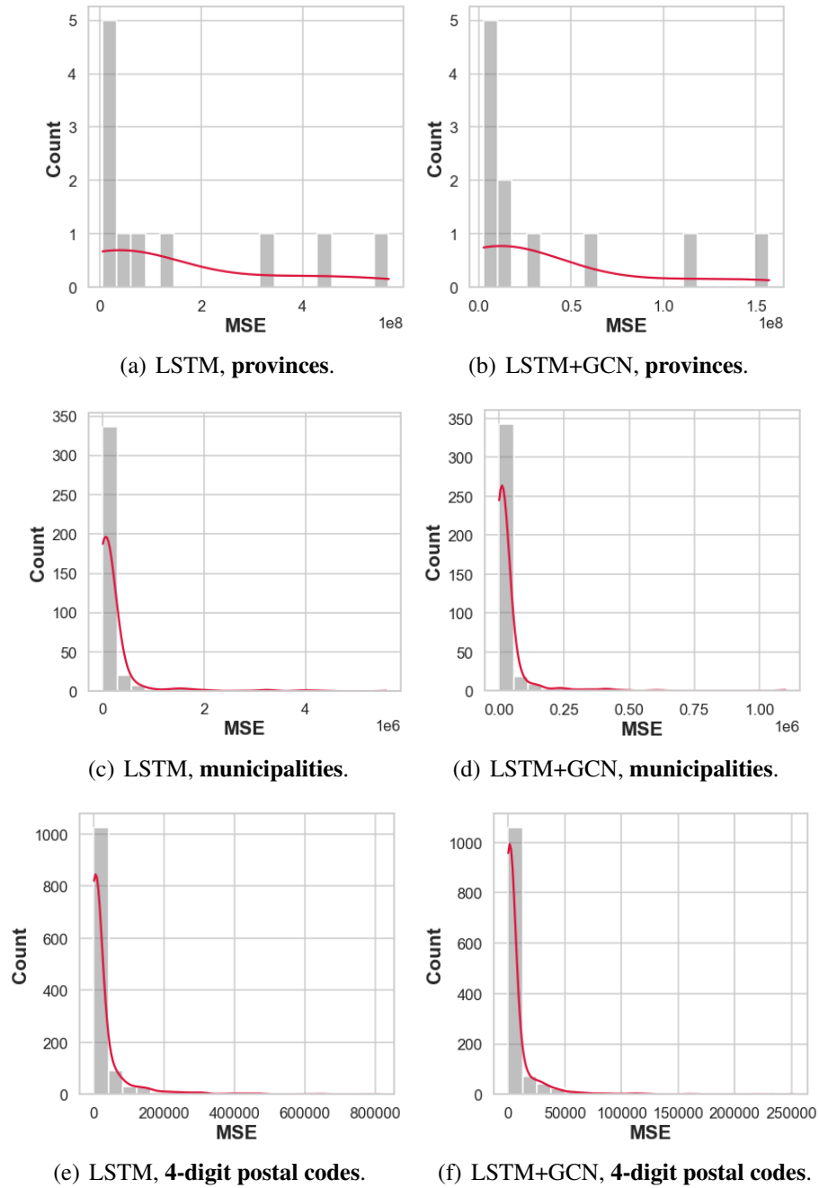
Figure 4.9: MSE for actual versus predicted trip production values per TAZ for each of the three spatial scales, using LSTM (left) and LSTM+GCN (right) model.
