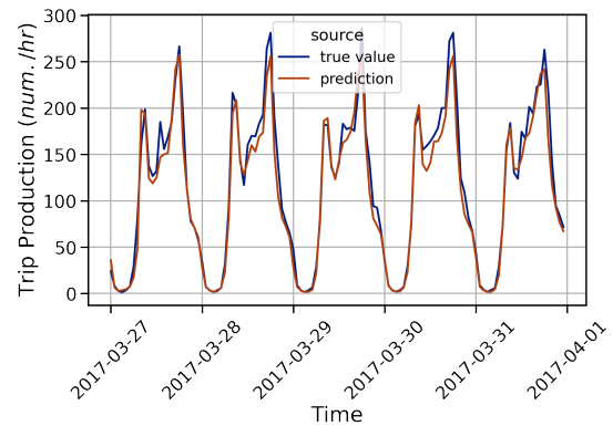
(e) 4-digit postal code zone prediction ( De Steeg e.o. ) with LSTM model.
