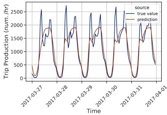
(c) Municipality prediction ( Rhenen ) with LSTM model.
