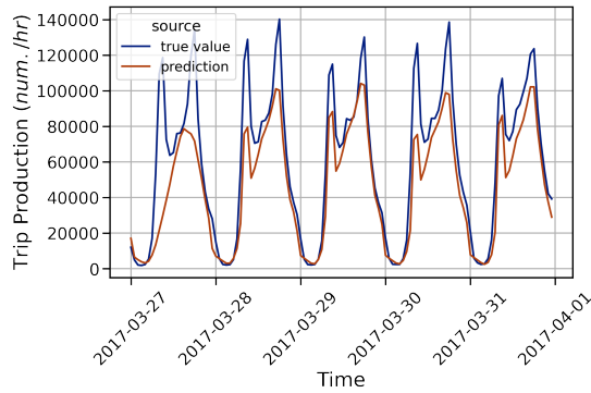
(a) Province prediction ( Gelderland ) with LSTM model.
