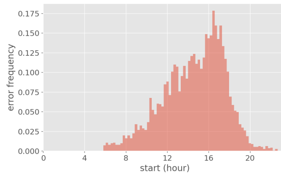
Figure 2.10: False negatives based on the start time of home.
