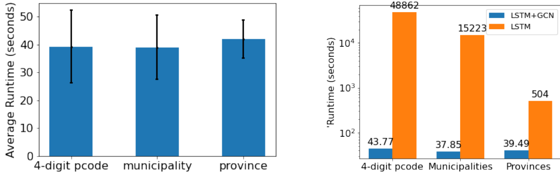
(a) Run time per TAZ of the LSTM model for the three spatial scales. (b) Total run time of the LSTM and LSTM+GCN model for the three spatial scales.
