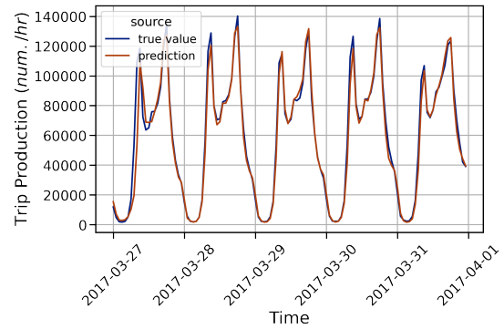
(a) Province prediction ( Gelderland ) with LSTM model.
