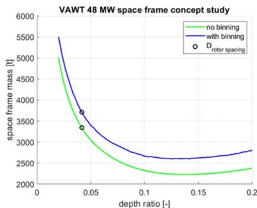
Figure 5. Space frame mass in relation to the space frame depth ratio
