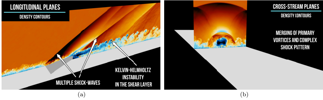
FIG. 4. Density contours on (a) longitudinal and (b) cross-stream planes.
