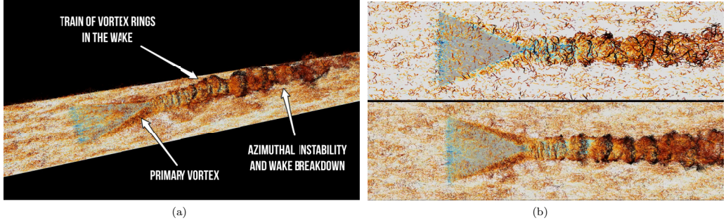
FIG. 2. Swirling strength isosurfaces coloured by streamwise velocity. (a) Main vortical structures at Re_\tau = 2000 . (b) Top view comparison of Re_\tau = 500 (top) and 2000 (bottom).
