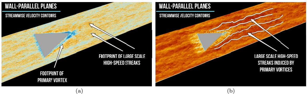
FIG. 3. Streamwise velocity contours on wall-parallel planes. (a) y^+ = 15 . (b) y/\delta = 0.3 .
