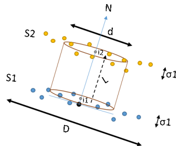
Figure 10. Illustration of M3C2 concept
