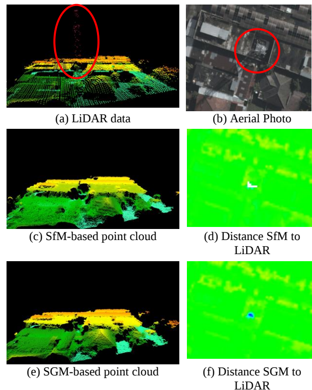
Figure 12. The communication tower in LiDAR and the M3C2 distance to image-based matching point
