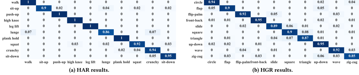
Figure 10: Confusion matrices of the classification results of ten human activities (HAR) and ten hand gestures (HGR).
