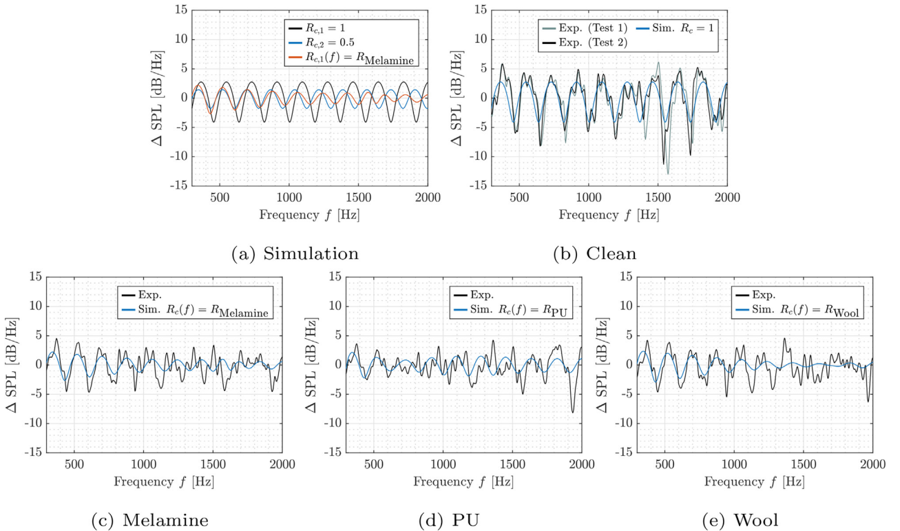
Fig. 10. Acoustic interference caused by a reflection vs. frequency, for a receiver located at the centre of the array (microphone 41). Comparison of simulations, considering different reflections: R_{c,1} = 1, R_{c,2} = 0.5 and R_{c,1}(f) = R_{\text{Melamine}} (top-left). Clean plate, measurement and simulation, considering R_c = 1 (top-right). Lined plates, measurement and simulation, considering R_{c,1} = R_{\text{Foam}} (bottom). Reflection coefficient of the lined plates obtained from experimental impedance tube data. Flow-off case, U_\infty = 0 \text{ ms}^{-1} .
