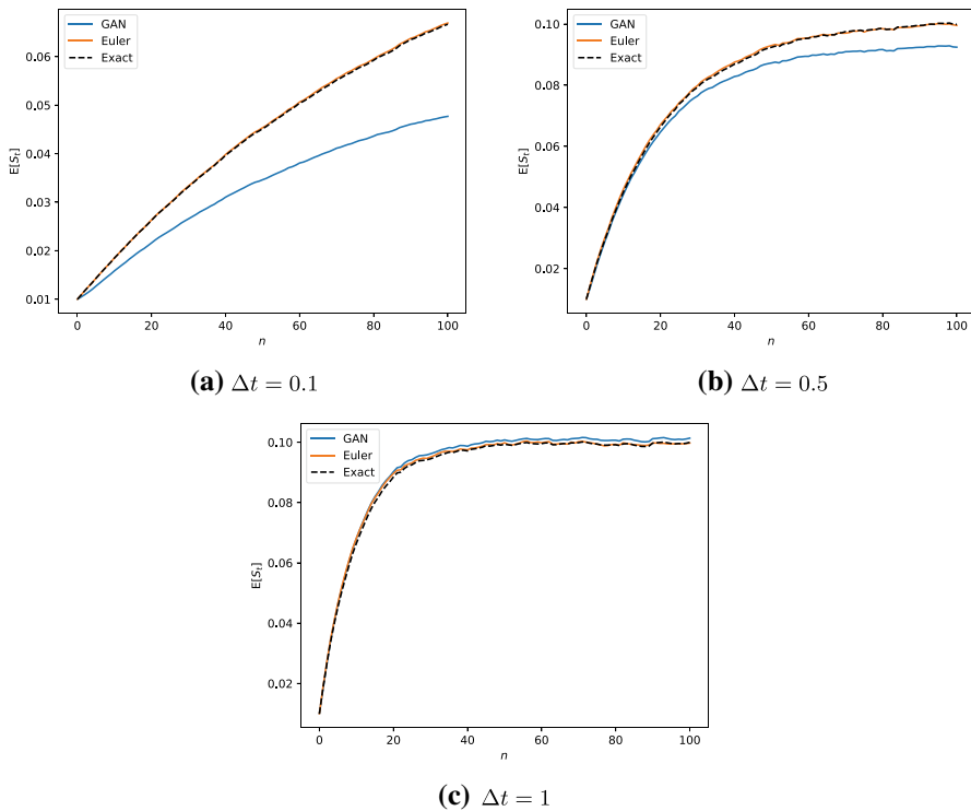
Fig. 4 Mean of 10^5 paths obtained with the supervised GAN after n repetitions of G_\theta(Z, S_t, \Delta t) , starting from S_0 = 0.01 . The mean reversion parameter was set to \bar{S} = 0.1 . The paths generated by the supervised GAN indeed exhibit mean reversion, although the GAN does not revert to the correct mean for every \Delta t . As \Delta t decreases, the error in the mean to which the GAN samples revert increases. This shows that the approximation of the conditional distribution is less accurate for smaller \Delta t , in line with our remaining benchmarks
