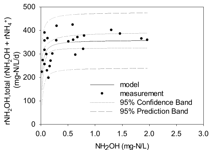
Fig. 5. Estimations of apparent kinetic parameters for ammonium oxidation by fitting Eq. (15) to the data from effluent hydroxylamine residual concentration over total ammonium oxidation consumption (hydroxylamine and ammonium) during continuous long term feeding.
