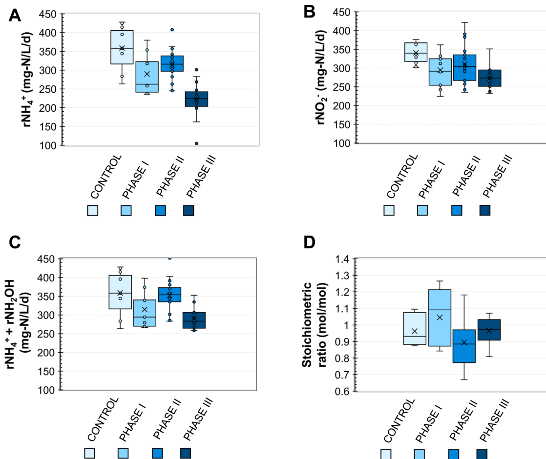
Fig. 3. Airlift reactor conversion rates and stoichiometric ratios for different hydroxylamine loading rates. A) Ammonium consumption rate, B) Nitrite production rate, C) Sum of ammonium and hydroxylamine consumption rate, D) Stoichiometric ratio of nitrogen produced over nitrogen consumed taking into hydroxylamine consumption.
