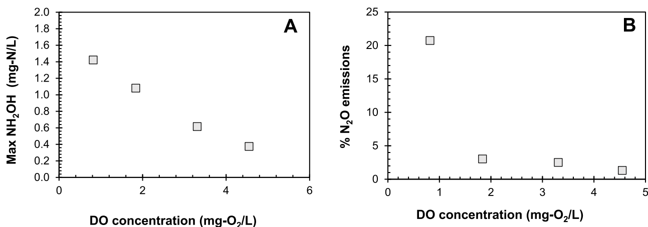
Fig. 2. Nitrification tests with ammonium present and continuous hydroxylamine feeding with granular sludge (biomass from reactor R2). Impact of dissolved oxygen concentration on: (A) Maximum accumulated hydroxylamine concentration (total amount added was between 7.4 to 3.5 mg-N/L, depending on the duration of the test) and (B) \text{N}_2\text{O} emissions as percentage of the total \text{N}_2\text{O} emitted over the total nitrogen consumed (ammonium + hydroxylamine).
