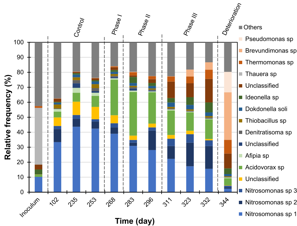
Fig. 4. Microbial relative frequency based on 16S rRNA sequencing of the predominant OTUs during different days of the airlift reactor operation.
