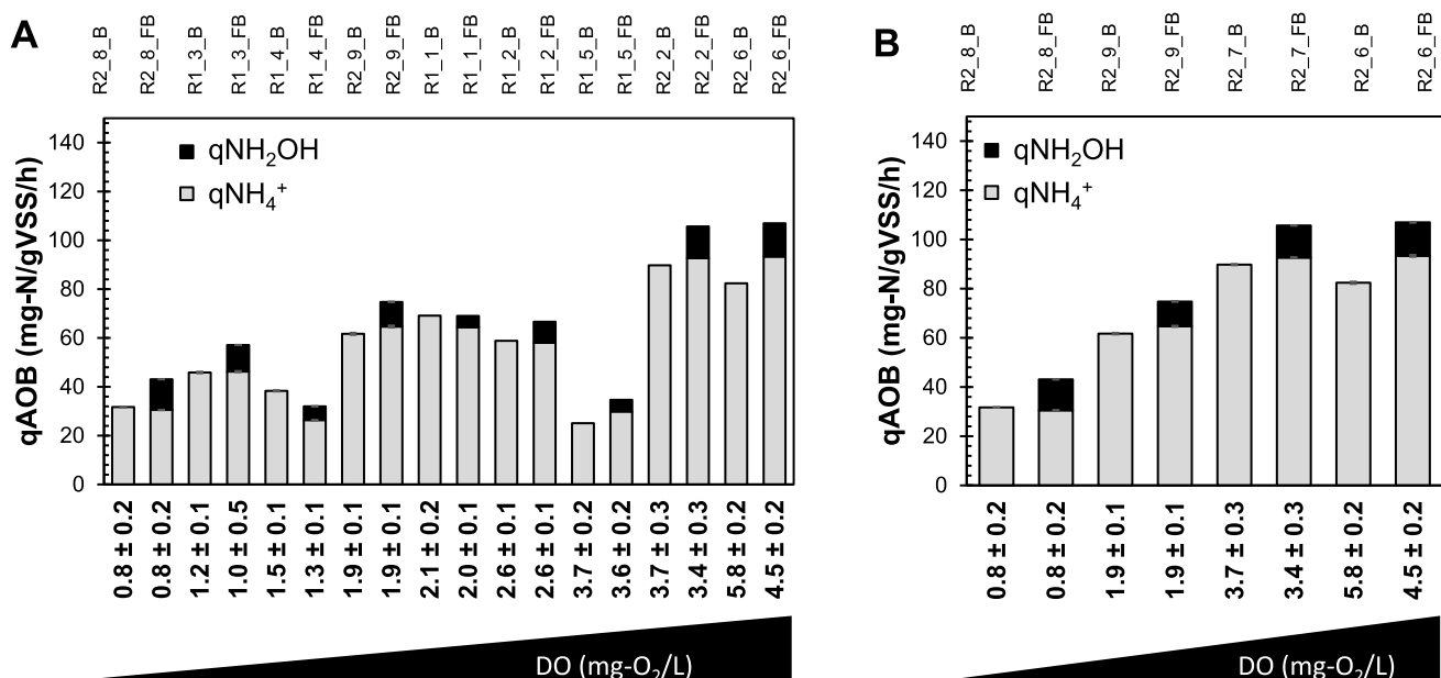
Fig. 1. Tests results performed with biomass from either inoculation period 1 (R1) or 2 (R2) followed by the number that corresponds with test conditions in Table 1. All respirometer tests consisted of an initial batch test (B) with only ammonium followed by a fed-batch (FB) with ammonium batch addition combined with hydroxylamine fed-batch. 9A) Comparison of all tests performed batch and fed-batch ammonium oxidation activity specific activity (qAOB), it is the addition of ammonium oxidation specific activity ( q_{\text{NH}_4^+} ) and hydroxylamine oxidation specific activity ( q_{\text{NH}_2\text{OH}} ) sorted by increasing conditions of oxygen. (B) Comparison of batch and fed-batch tests performed with biomass from R2, sorted in increasing dissolved oxygen concentrations.
