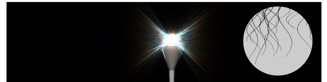
Figure 14: An example glare rendering with an eyelash aperture.
