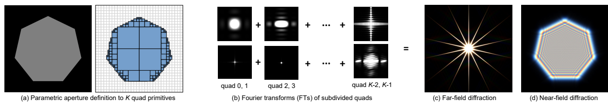
Figure 1: Given an aperture image, we subdivide it into a list of parametric quad primitives forming a quadtree (a). The Fourier transform of each quad is efficiently evaluated with a closed-form solution (b), and combined to render the final far-field diffraction (c). We extend this approach to also produce near-field diffraction (d). (c) and (d) are rendered in 0.85 ms and 2.1 ms at 1024 \times 1024 resolution, respectively.
