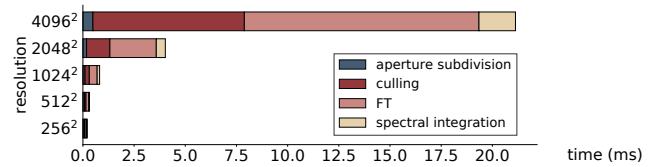
Figure 11: Per-stage performance breakdown of our FFD rendering for the Heptagon aperture.
