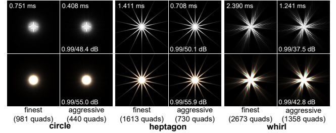
Figure 9: Comparison of quality in terms of quadtree resolution for monochromatic and dispersive FFDs. The one-step further down-sampling from the finest quadtree resolution results in a negligible visual difference (SSIM/PSNR at the bottom), while increasing speed by a factor of two (timings given at the top).
