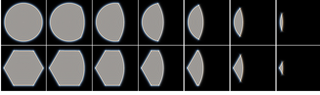
Figure 15: The dynamic ringing of the aperture cropped by the lens housing, which can be used for realistic lens-flare rendering.
