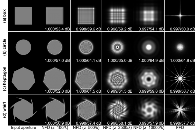
Figure 8: FFD and NFD outputs (scaled for illustration) for the input aperture images (the first column) used for the experiment. The numbers at the bottom indicate SSIM/PSNR values measured against the references (generated by discrete NFD/FFD solutions).
