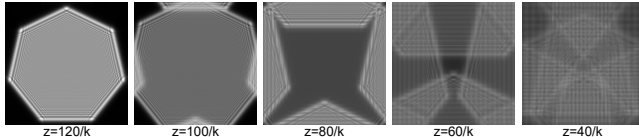
Figure 12: As z decreases, the discrete NFD without enough zero padding leads to interference patterns. Our NFD solution does not suffer from these artifacts.
