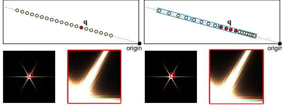
Figure 4: Uniform spectral scaling (left) and 4-channel batch spectral scaling (right), with examples for the diffraction of an hexagonal aperture. Our batch scaling saves the amount of lookups from the base pattern by roughly a factor of four.
