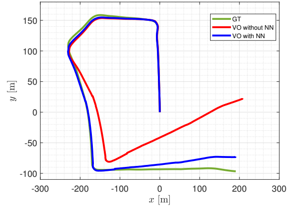
Fig. 5. The computed trajectory by the VO with and without the DRNN along with the ground-truth trajectory of the testing portion of sequence 5 of KITTI dataset.
