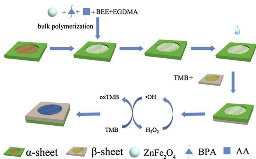
Figure 6. Construction of a paper-based MIP assay for the detection of BPA in liquid. Figure reproduced from [126] with permission from copyright Elsevier 2017.
