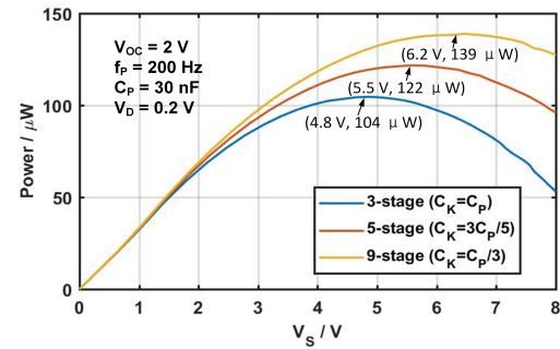
Fig. 7. Simulated output power of 3-, 5- and 9-stage SSHC with equal total capacitance ( C_{total} = 3C_P ) but different phase schedules.
