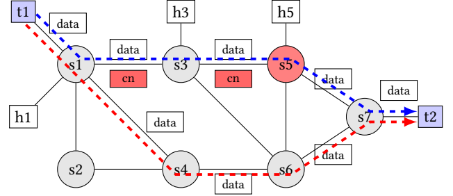
Figure 5: If switch s5 is congested, no better route can be found to t2. In this case, s5 will send a packet to s3 informing s3 not to send packets through s5. S3 forwards this control packet to s1, who will consequently reroute the traffic to s4.
