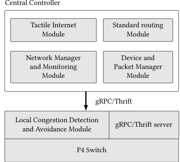
Figure 1: Hierarchical design of the control plane.
