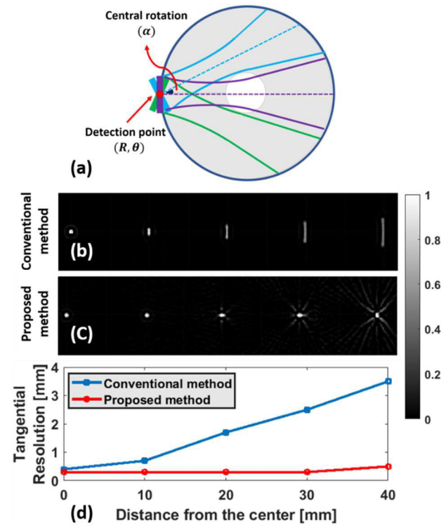
Fig. 1: (a) Schematic of the proposed detection approach. The reconstructed images with (b) the conventional and (c) the proposed method using point targets. (d) The tangential resolution for different off-center distances.
