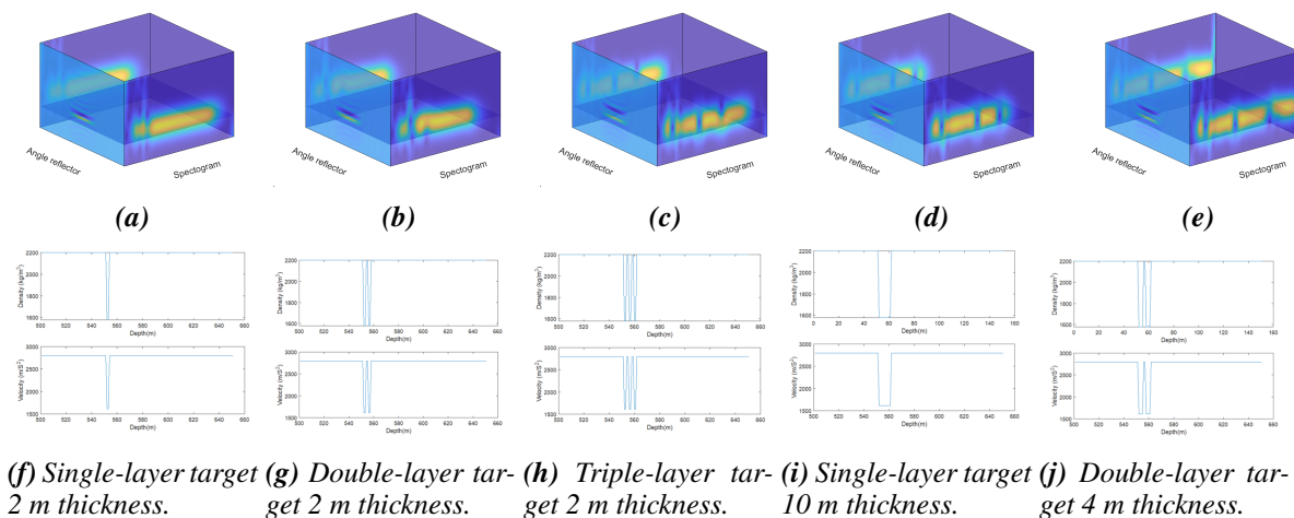
Figure 5: The spectrogram patterns for various target-layer-setting with corresponding density and velocity structure.
