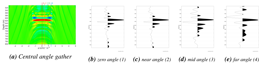
Figure 3: (a) Subsurface angle gather for a single 2-meter thickness target layer obtained after the FWM step for the central location. (b) trace for ray parameter 0, (c,d,e) traces for near-, mid- and far-angle ray parameters.
