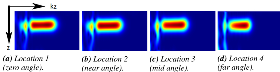
Figure 4: Spectrogram for different ray-parameter in Figure 3.
