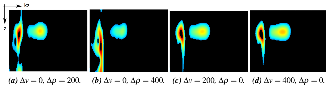
Figure 2: Mid-angle gather spectrogram changes for a single layer with thickness 2 meter; the \Delta v -values are in m/s, the \Delta \rho -values in \text{kg/m}^3 .
