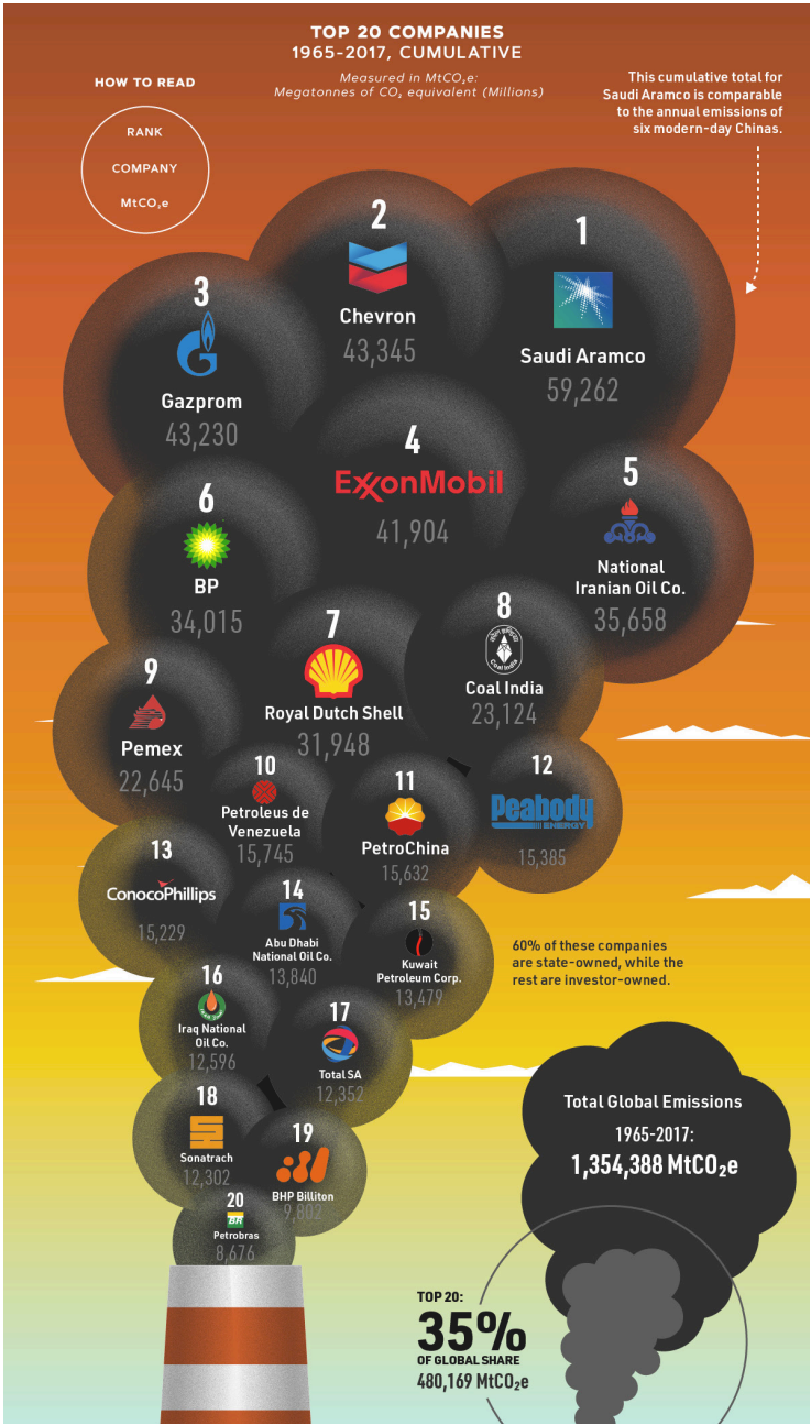
(above) The companies responsible for the most global carbon emissions. The illustration show that just 20 companies are responsible to contribute over a third of all carbon emissions since 1965. A switch to low-carbon technologies is crucial. Image 7: Visual Capitalist, 2021
