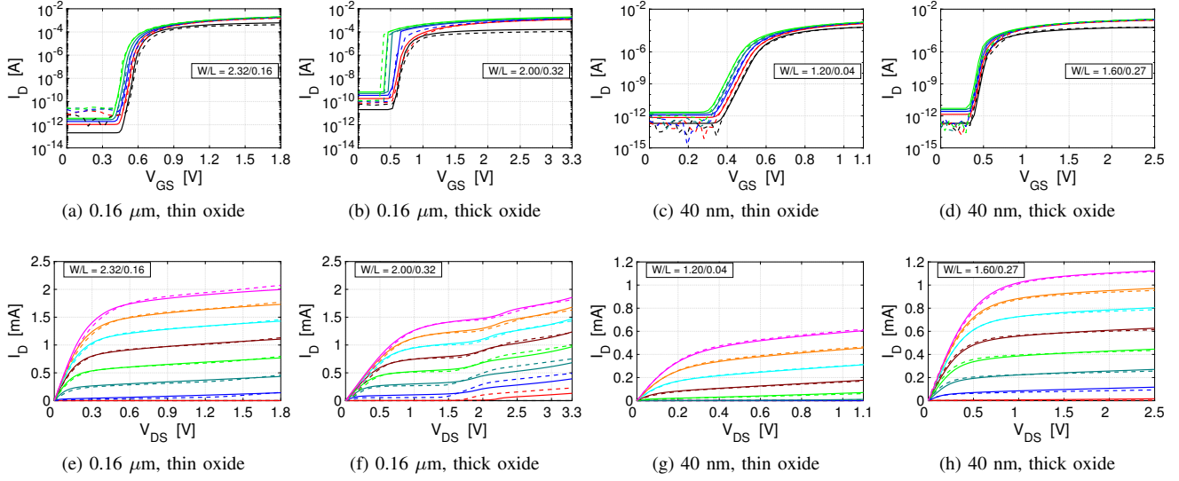
Fig. 15. Models (solid) and measurements (dashed) at 4 K; W/L in \mu\text{m} . (a,e) I_D(V_{GS}) and I_D(V_{DS}) of 0.16- \mu\text{m} thin-oxide NMOS; (b,f) I_D(V_{GS}) and I_D(V_{DS}) of 0.16- \mu\text{m} thick-oxide NMOS; (c,g) I_D(V_{GS}) and I_D(V_{DS}) of 40-nm thin-oxide NMOS; (d,h) I_D(V_{GS}) and I_D(V_{DS}) of 40-nm thick-oxide NMOS.
