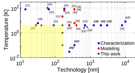
Fig. 1. Summary of CMOS technologies measured at cryogenic temperatures. The works on characterization are indicated by blue squares while attempts at modeling by red diamonds. The references with an asterisk showed kink.
