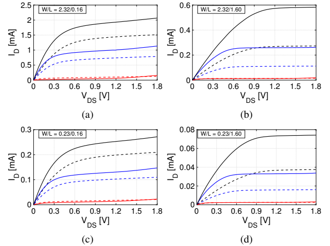
Fig. 3. Measured I_D(V_{DS}) characteristics of thin-oxide NMOS in 0.16- \mu\text{m} CMOS. V_{GS} = [0.68 \text{ V}; 1.24 \text{ V}; 1.8 \text{ V}] . Solid line: 4 K; dashed line: 300 K.
