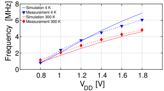
Fig. 17. Ring oscillator frequency versus supply voltage ( V_{DD} ) at 300 K and 4 K. Measurements (dotted lines) and simulations (solid lines) are compared with the compact model presented in Section IV.
