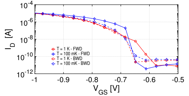
Fig. 13. Forward (FWD) and backward (BWD) sweep of I_D(V_{GS}) for the thin-oxide PMOS ( 2.32/1.6 ) at 1 K and 100 mK at V_{DS} = -1.8 V.
