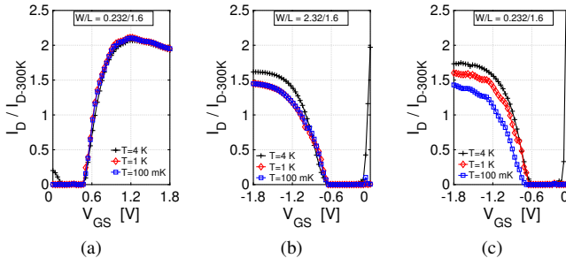
Fig. 10. Measured characteristics of the three devices tested at 1 K and 100 mK compared to 4 K; (a) NMOS, V_{DS} = 1.8 \text{ V} ; (b)-(c) PMOS, V_{DS} = -1.8 \text{ V} . Every curve is normalized to 300 K to remove chip-to-chip spread since the 4 K measurements were done on a different chip placed in the probe station.
