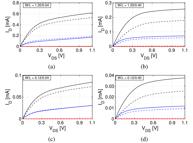
Fig. 7. Measured I_D(V_{DS}) characteristics of thin-oxide NMOS in 40-nm CMOS. V_{GS} = [0.43 \text{ V}; 0.76 \text{ V}; 1.1 \text{ V}] . Solid line: 4 K; dashed line: 300 K.
