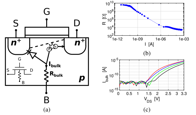
Fig. 11. (a) Cross-Section and schematic representation of the cause of kink effect at 4 K; (b) N-well resistance versus current at 4 K; the resistance value at 300 K is 3.5 kΩ; (c) I_{bulk}(V_{DS}) of thick-oxide NMOS, W/L = 2.32/0.322 at 4 K.
