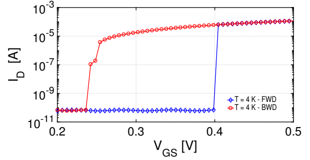
Fig. 12. Forward (FWD) and backward (BWD) sweep of I_D(V_{GS}) in subthreshold region for the thick-oxide NMOS ( W/L = 2.32/0.16 ) at 4 K at V_{DS} = 3.3 V. Hysteresis causes a shift of \approx 0.15 V.
