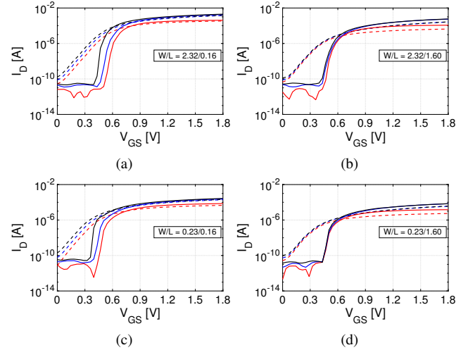
Fig. 2. Measured I_D(V_{GS}) characteristics of thin-oxide NMOS in 0.16- \mu\text{m} CMOS. V_{DS} = [0.1 \text{ V}; 0.95 \text{ V}; 1.8 \text{ V}] . Solid line: 4 K; dashed line: 300 K.
