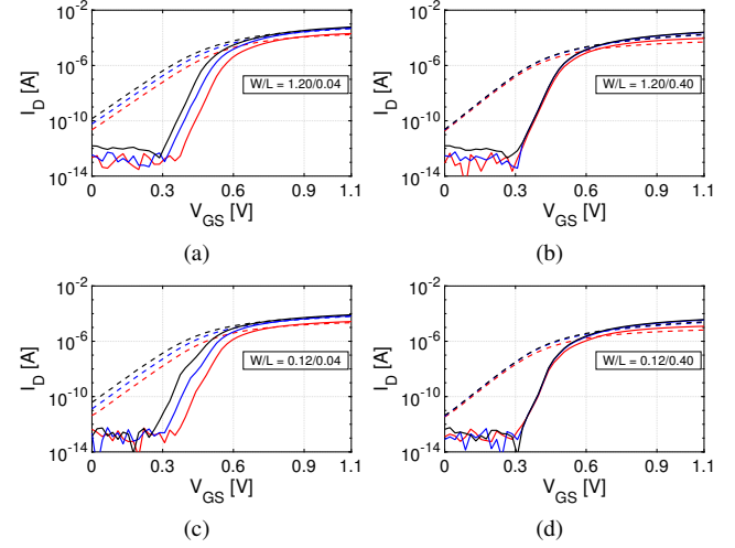
Fig. 6. Measured I_D(V_{GS}) characteristics of thin-oxide NMOS in 40-nm CMOS. V_{DS} = [0.1 \text{ V}; 0.6 \text{ V}; 1.1 \text{ V}] . Solid line: 4 K; dashed line: 300 K.
