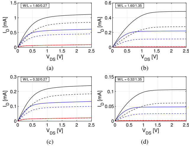
Fig. 9. Measured I_D(V_{DS}) characteristics of thick-oxide NMOS in 40-nm CMOS. V_{GS} = [0.85 \text{ V}; 1.68 \text{ V}; 2.5 \text{ V}] . Solid line: 4 K; dashed line: 300 K.
