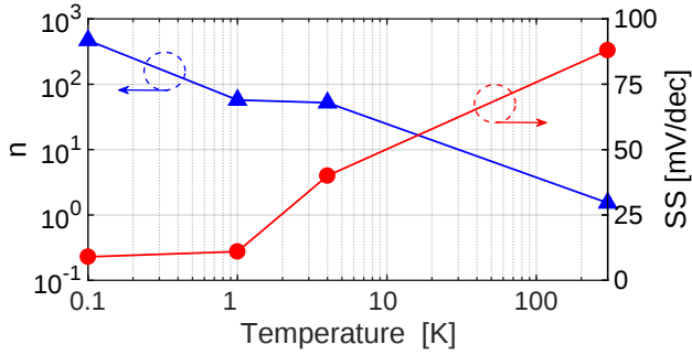
Fig. 14. Subthreshold slope ( SS ) and extracted ideality factor n of the PMOS ( W/L = 2.32/1.6 ) across temperature.
