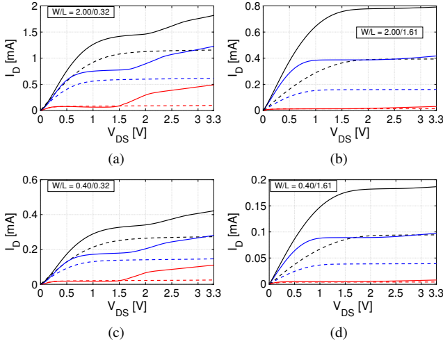
Fig. 5. Measured I_D(V_{DS}) characteristics of thick-oxide NMOS in 0.16- \mu\text{m} CMOS. V_{GS} = [1.05 \text{ V}; 2.17 \text{ V}; 3.3 \text{ V}] . Solid line: 4 K; dashed line: 300 K.
