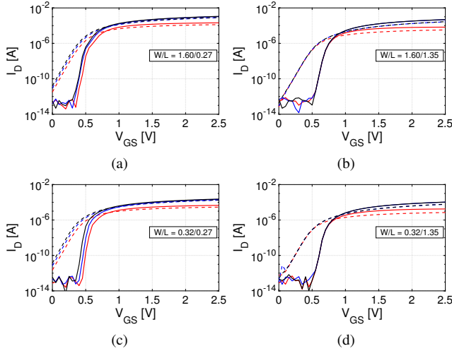
Fig. 8. Measured I_D(V_{GS}) characteristics of thick-oxide NMOS in 40-nm CMOS. V_{DS} = [0.1 \text{ V}; 1.3 \text{ V}; 2.5 \text{ V}] . Solid line: 4 K; dashed line: 300 K.
