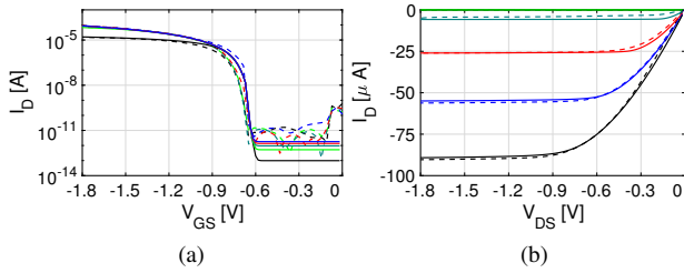
Fig. 16. Models (solid) and measurement (dashed) of 0.16- \mu\text{m} thin-oxide PMOS (W/L = 2.32/1.6) at 100 mK. (a) I_D(V_{GS}) , V_{DS} = -1.8 \rightarrow -0.09 V; (b) I_D(V_{DS}) , V_{GS} = -0.3 \rightarrow -1.8 V.
