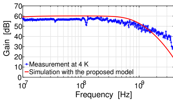
Fig. 18. Frequency response of the cryogenic LNA: comparison between measurement at 4 K and simulation with the proposed model. Reproduced from [42].
