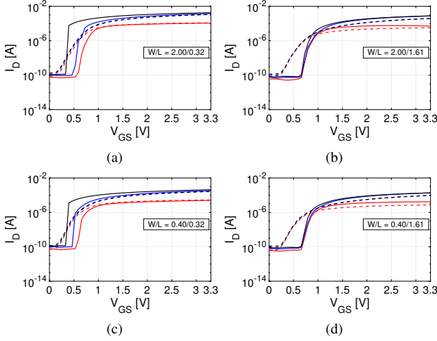
Fig. 4. Measured I_D(V_{GS}) characteristics of thick-oxide NMOS in 0.16- \mu\text{m} CMOS. V_{DS} = [0.1 \text{ V}; 1.7 \text{ V}; 3.3 \text{ V}] . Solid line: 4 K; dashed line: 300 K.
