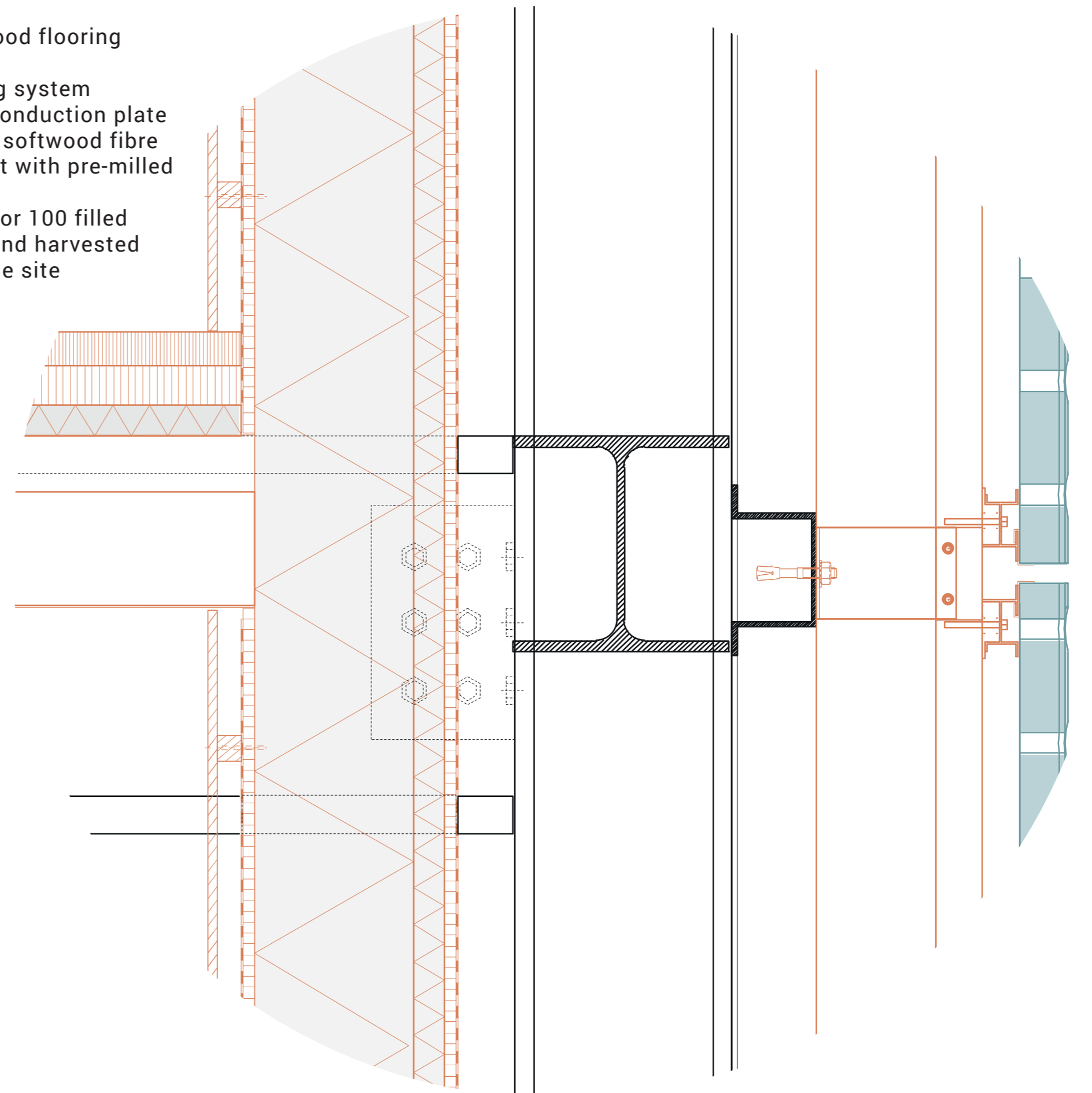
DETAIL D 1:5
