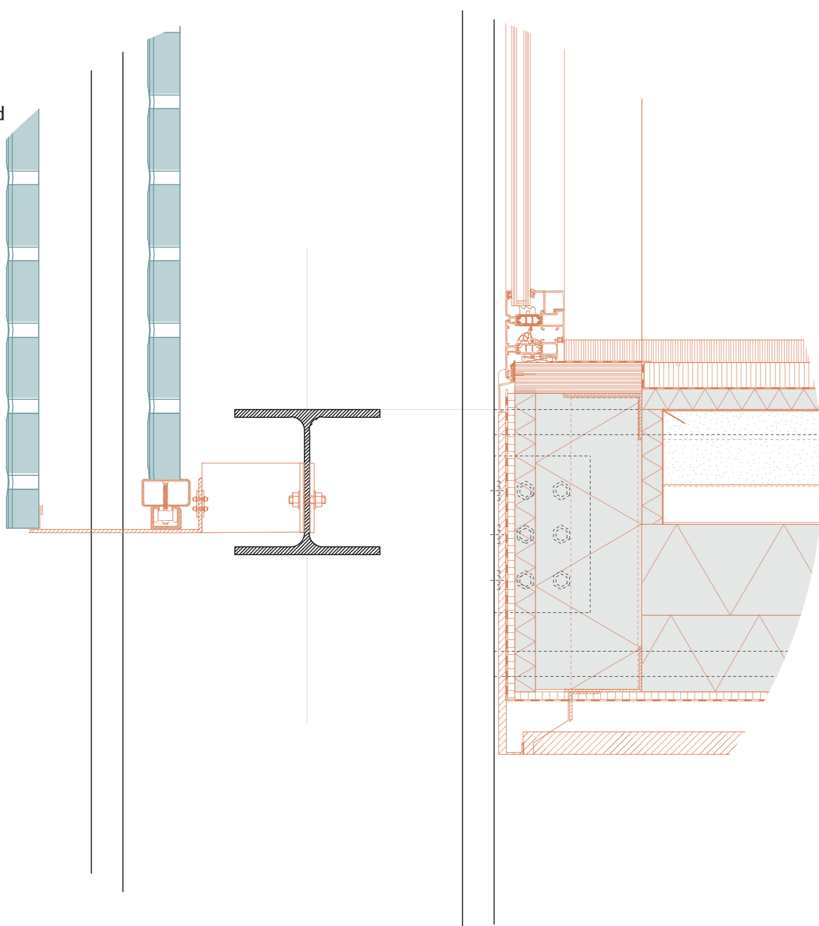
DETAIL F 1:5
