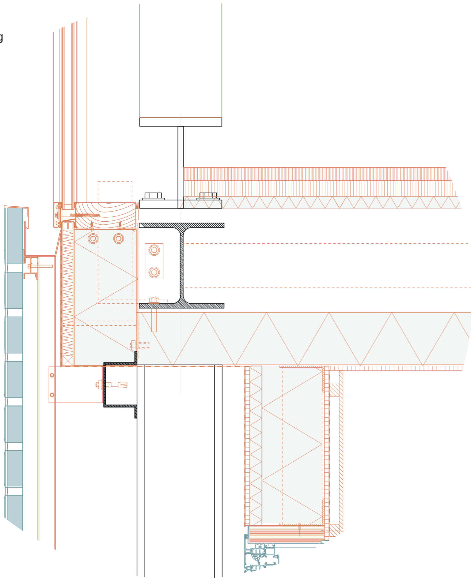
DETAIL D 1:5
