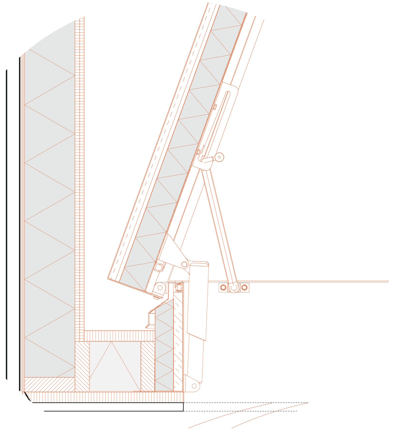
DETAIL B 1:5 Entrance Silo Room
