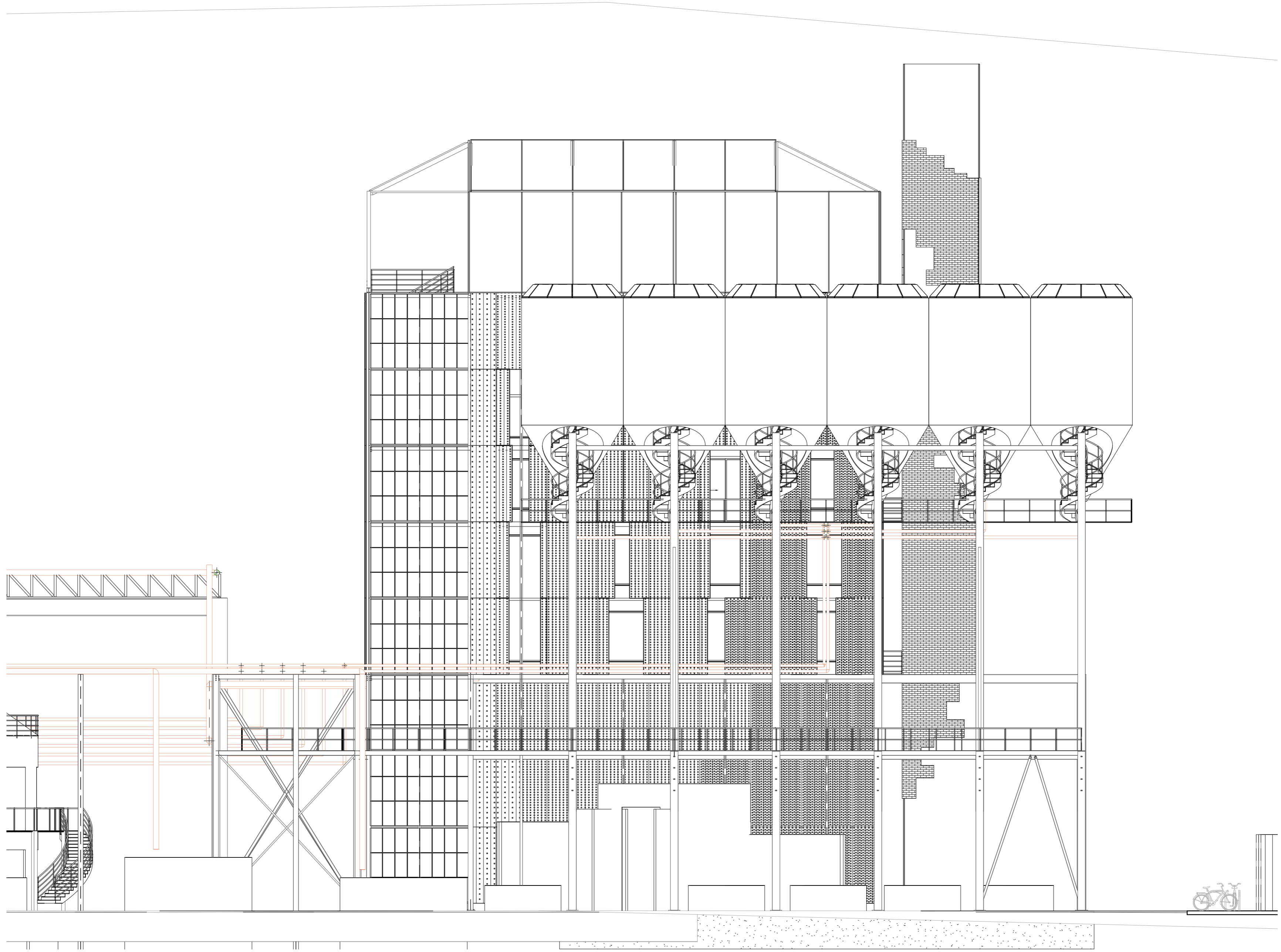
SOUTH FACADE Flexible facade
