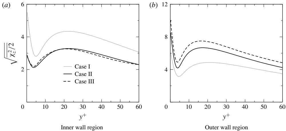
FIGURE 16. R.m.s. values of the streamwise momentum vorticity in the near-wall regions in the reference case (I), forced convection s\text{CO}_2 case (II) and mixed convection s\text{CO}_2 case (III).
