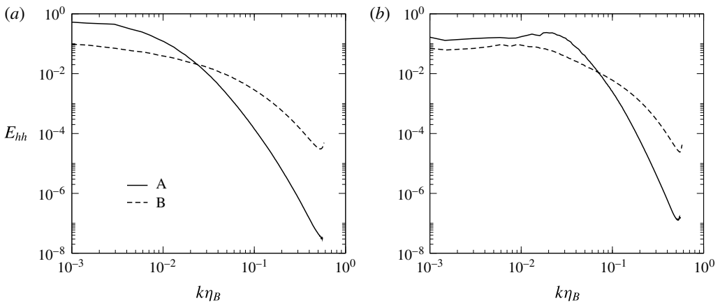
FIGURE 23. (a) Streamwise and (b) circumferential power spectra of enthalpy fluctuations. Curve A corresponds to the location where h_{rms} is largest, and curve B refers to the location where \bar{Pr} is largest.
