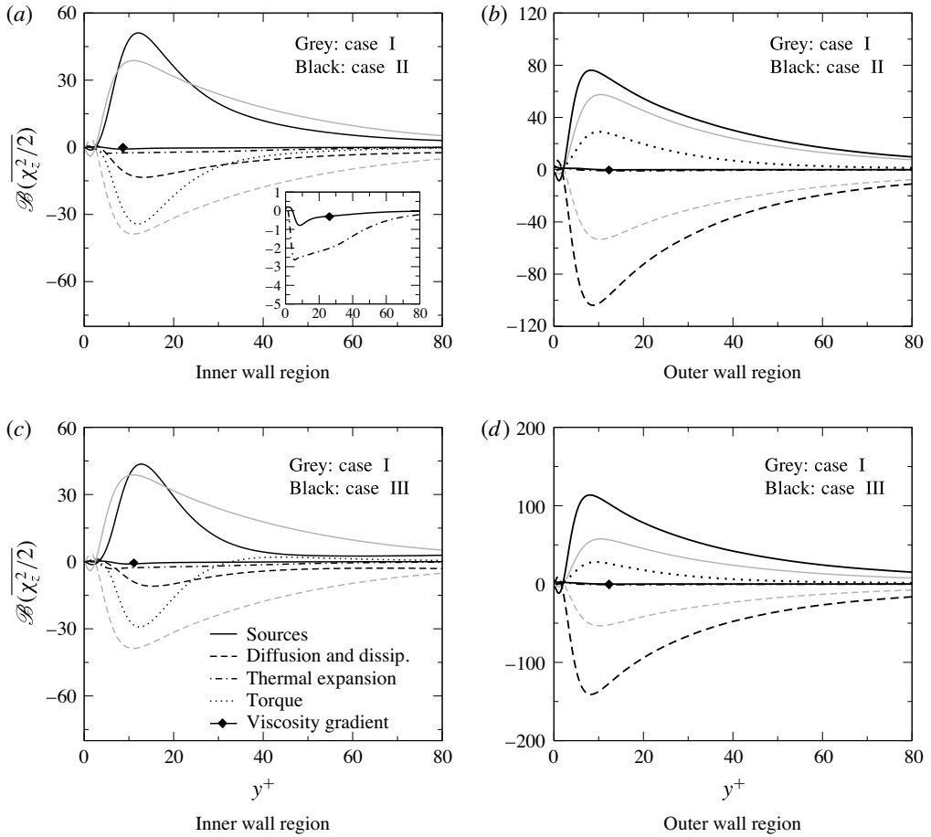
FIGURE 17. Budgets of the streamwise vorticity \mathcal{B}(\overline{\chi_z^2/2}) , equation (3.12). Black lines are used for the forced convection (II) and mixed convection (III) sCO 2 cases, while grey lines are reserved for the reference case (I).
