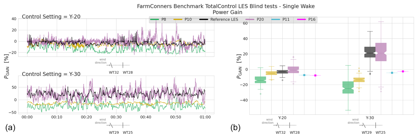
Figure 23. TotalControl LES blind tests, power gain, P_{\text{GAIN}} , estimations for single wake under wake steering for the two-turbine configurations with 5 D spacing (WT32–WT28 with 20° yaw and WT29–WT25 with 30° yaw at the upstream turbines). (a) Time series of P_{\text{GAIN}} , illustrated at the submitted frequency by the participants, for both control scenarios. (b) The distribution of the P_{\text{GAIN}} within the 1 h blind test period for both 20 and 30° anticlockwise yaw misalignment WFFC scenarios.
