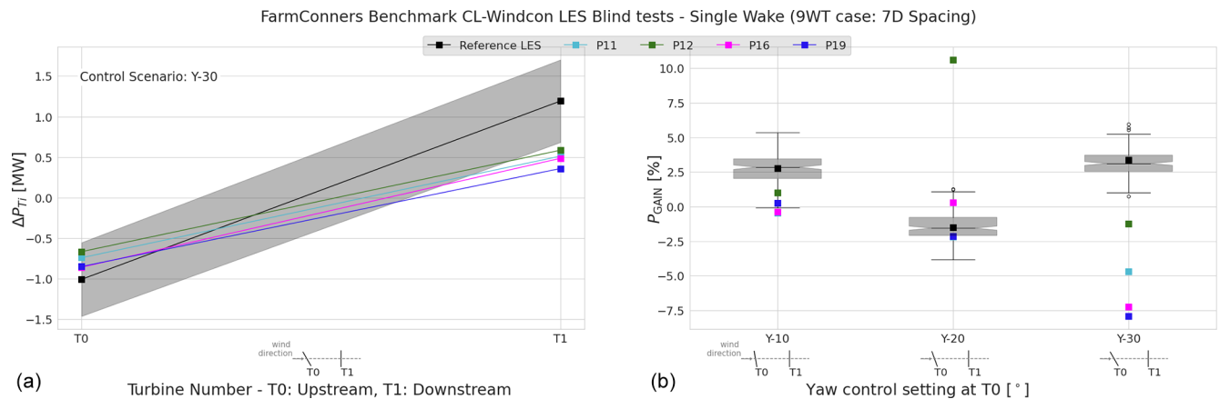
Figure 17. CL-Windcon LES blind tests, single wake under wake steering for the nine-turbine configuration (9WT) with 7 D spacing. (a) Power difference (mean) in absolute values (MW) per upstream (T0) and downstream (T1) turbine, when T0 is -30^\circ misaligned (Y-30). (b) Power gain (mean) for the two-turbine subset of the wind farm (T0 + T1). Boxplots represent the distribution of the reference CL-Windcon LES time series per control settings where T0 is misaligned -10^\circ (Y-10), -20^\circ (Y-20), and -30^\circ (Y-30). Representative layouts with corresponding yaw control settings are illustrated along the x axes.
