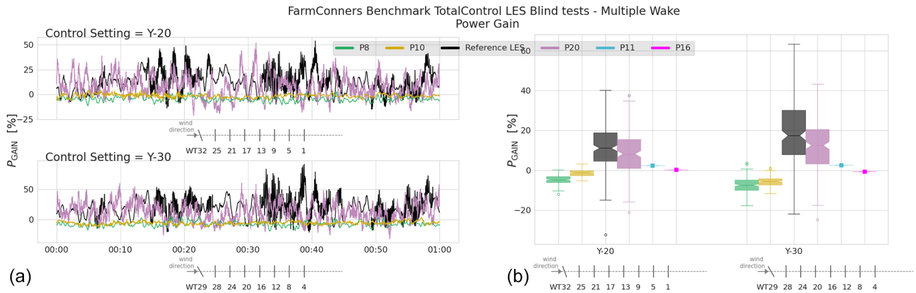
Figure 24. TotalControl LES blind tests, power gain estimations, P_{\text{GAIN}} , for multiple wakes under the upstream wake steering for the eight-turbine configurations with 5 D spacing (WT32–WT4 with 20° yaw and WT29–WT1 with 30° yaw at the upstream turbines). (a) Time series of P_{\text{GAIN}} , illustrated at the submitted frequency by the participants. (b) The distribution of the P_{\text{GAIN}} within the 1 h blind test period, for both 20 and 30° anticlockwise upstream yaw misalignment WFFC scenarios.
