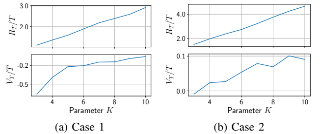
Fig. 4: Sensitivity of OLR-SO on K . We used T=1000 , B=10 . (4a): d=[20, 20, 20] , \nu=0.9 and \mu=0.03 . (4b): d=[5, 5, 5] , \nu=0.1 and \mu=0.01 .
