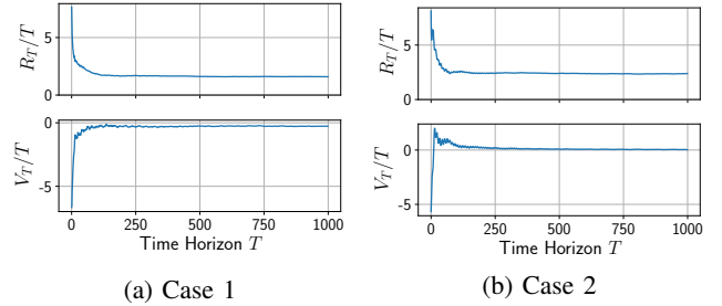
Fig. 3: Evolution of R_T/T and V_T/T for OLR-SO. We use T=1000 , K=5 , B=10 and d=3 . (3a): d=[20, 20, 20] , \nu=0.9 and \mu=0.03 . (3b): d=[5, 5, 5] , \nu=0.1 and \mu=0.01 .
